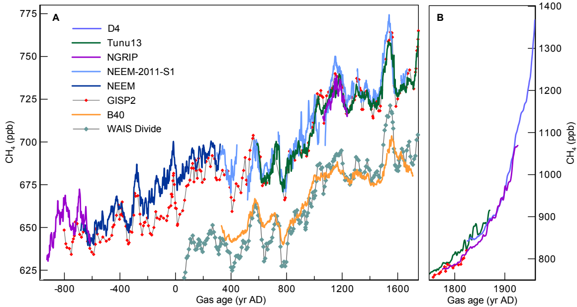
3 Figure 2. Late Holocene continuous CH 4 data from Tunu13, D4, NGRIP and NEEM 4 Greenland ice cores and B40 Antarctic ice core for time periods -900–1750 AD (A) and 5 1750–1960 AD (B). Each record is a cubic spline fit with 1 yr sample spacing to the 5 s 6 integrated data. No data from the lock-in zone are included on this figure. Also plotted 7 are discrete CH 4 data from GISP2 and WAIS Divide ice cores (Mitchell et al., 2013) and 8 NEEM-2011-S1 continuous CH 4 data (Rhodes et al., 2013).
