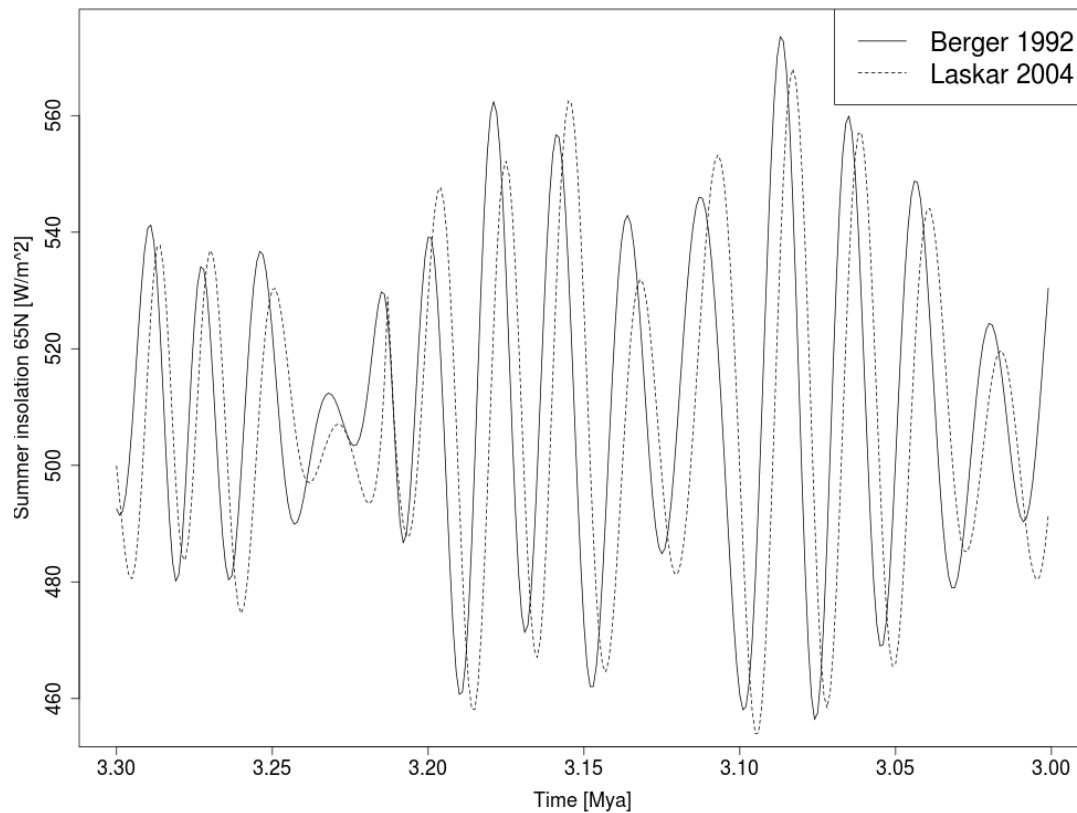
Fig. 1. Comparison of Laskar 2004 and Berger 1992 astronomical solutions in terms of the summer insolation at 65N for the mid-Pliocene interval.
