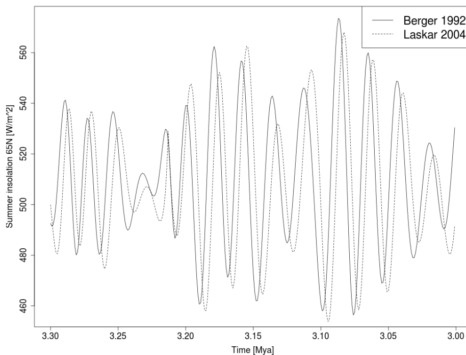
Fig. 1. Comparison of Laskar 2004 and Berger 1992 astronomical solutions in terms of the summer insolation at 65N for the mid-Pliocene interval.
