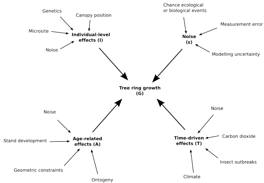
Supplementary Figure: A conceptual diagram of tree ring growth. The ultimate causes of tree growth (plain text) can be grouped according to the pattern of variability (common to each individual, time or age) they induce in tree-ring growth. By partitioning the observed variability in tree-ring growth into latent effects, we can separate time-driven effects (climate, CO 2 etc.) from age or individual-related effects. This "time effect" (common temporal signal) is the target of standardization, not "typical growth".
