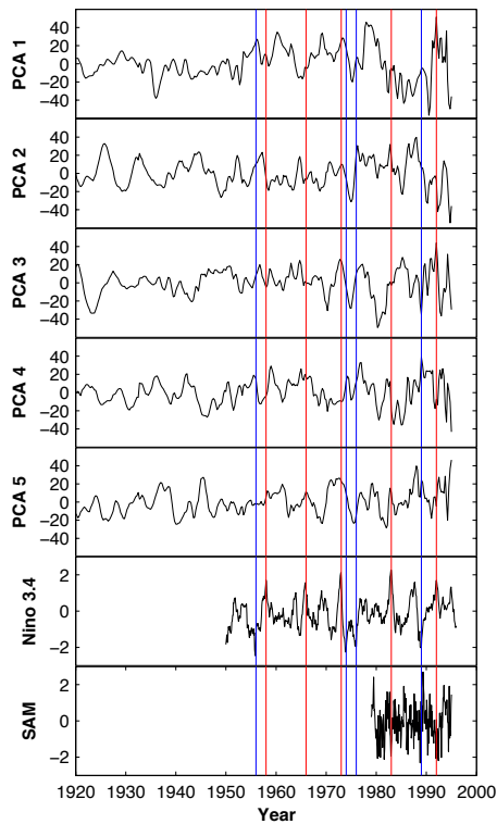
Fig. 8. First 5 principal components compared with strong El Niño years (red) and strong Niña years (blue), Nino 3.4 SST, and the SAM.
