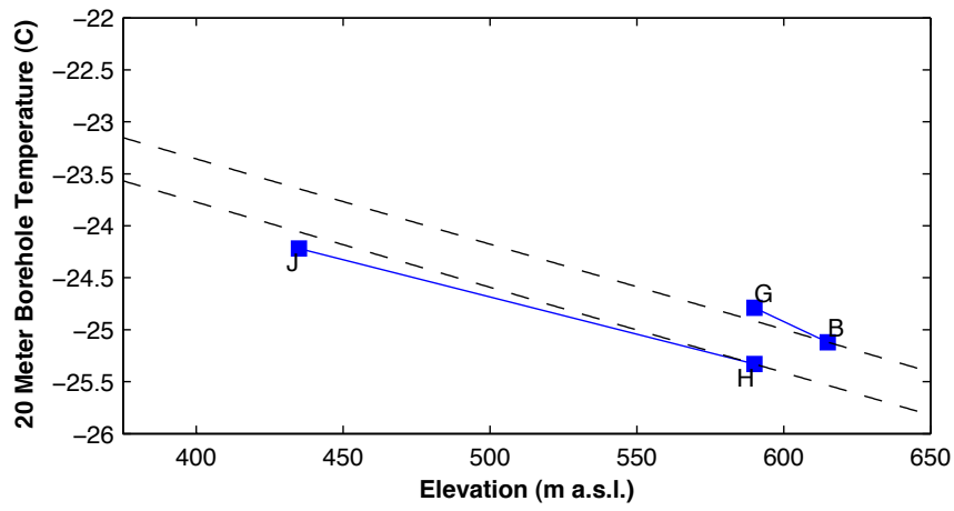
Fig. 3. Twenty-meter borehole temperatures.
