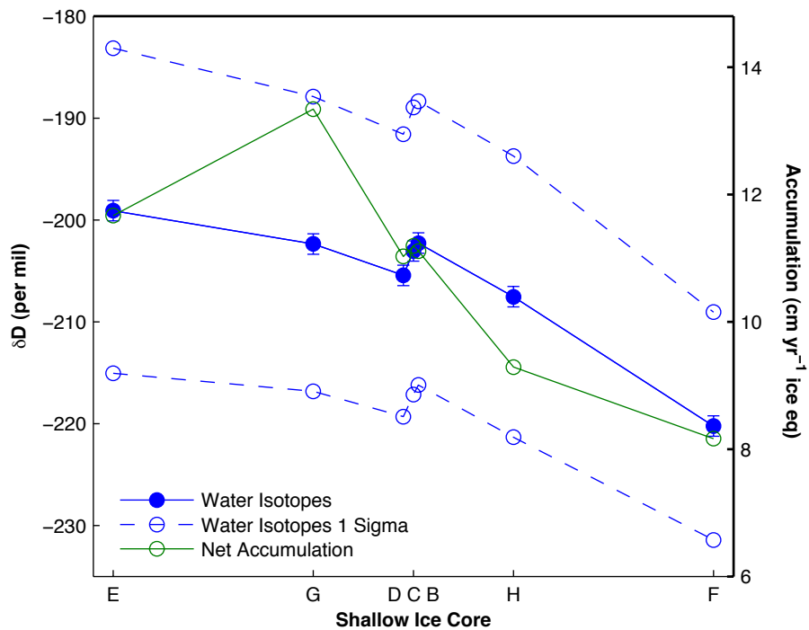
Fig. 2. Delta-D and Accumulation averages (1920-1995).
