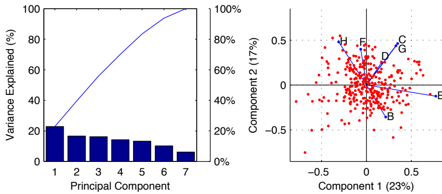
Fig. 7. PCA analysis of Siple Dome shallow ice cores, including the variance explained by each component, and a bi-plot of component 1 and 2.
