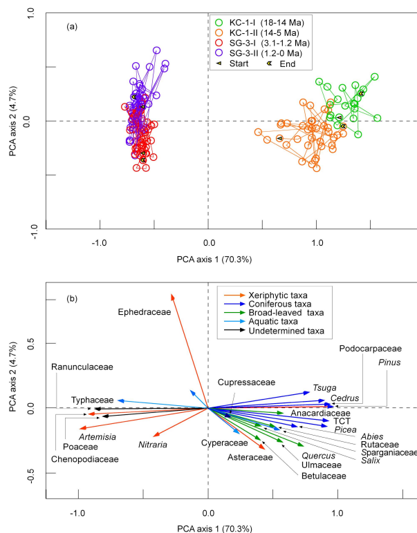
Fig. 1. Fig. 6 PCA-plot of samples and species
