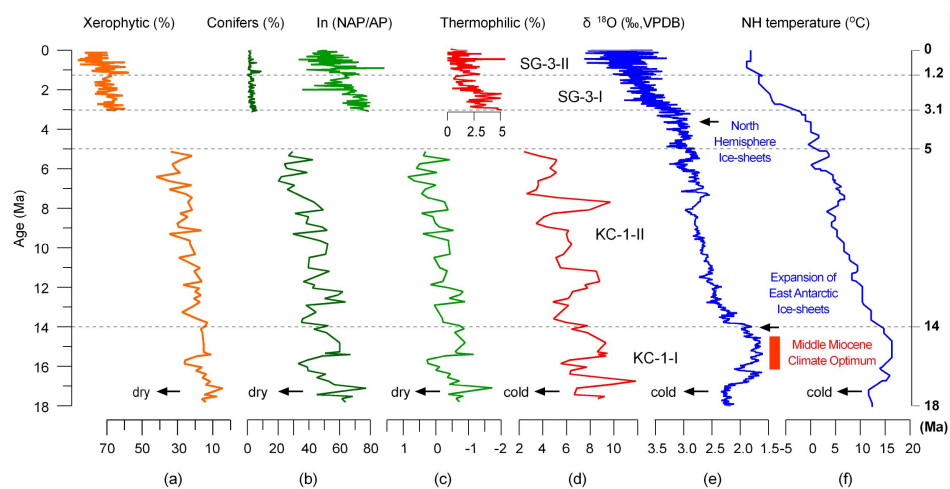
Fig. 2. Fig. 7 Comparison of xerophytic, conifer percentages, ln (NAP/AP) and global temperature
