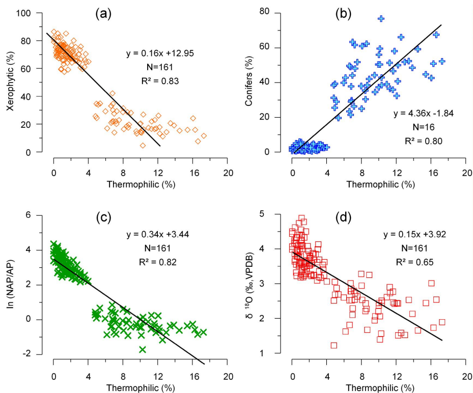
Fig. 3. Fig. 8. Correlation results between pollen and oxygen isotope data
