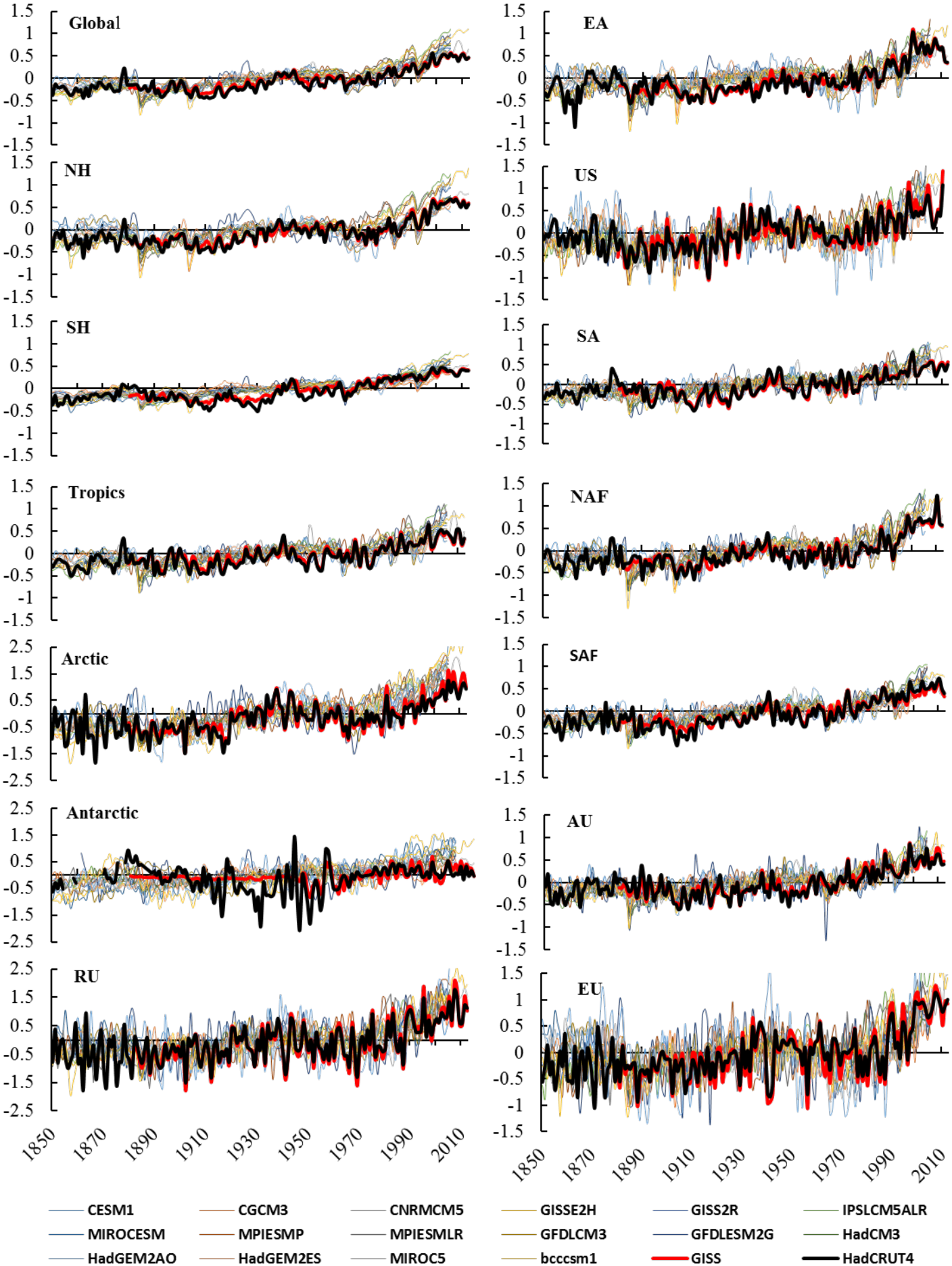
Fig. S1 The time series of annual mean surface temperature anomalies(°C) in the period of 1850-2012
