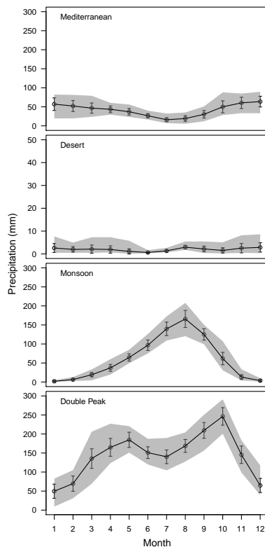
Fig. 1. Observed seasonal cycle of precipitation in each of the defined climate zones, using the CRU T3.1 data set (Harris et al., 2013). The mean precipitation each month (mm) is shown by the black line, with the standard deviation shown by the bars. The grey shading shows the maximum and minimum rainfall experienced within the observation period (1961–1990). Note that the scale for the desert region differs from that used for the other regions. Months are numbered consecutively from January (1) through to December (12).
