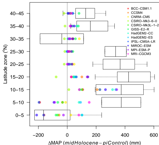
Fig. 7. Comparison of simulated and reconstructed changes in mean annual precipitation in the mid-Holocene for 5^\circ latitude bands between 0 and 45^\circ N. The reconstructions are from the Bartlein et al. (2011) data set. The mean, 25–75 % range and full range of the reconstructions are shown (for those latitude bands with sufficient data points). The model results are averages for the grid cells with observations.
