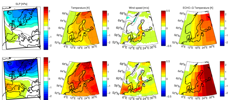
Fig. 3. The new figure 7 including patterns from ECHO-G.
