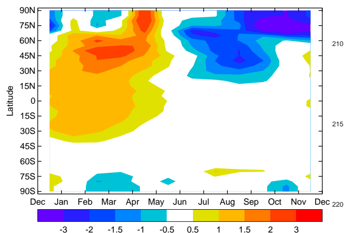
Fig. 1. Difference between 115 ka BP (incipient glacial) and recent conditions (IG minus recent) as a function of latitude and time of year in climatological surface air temperature in years 301–330 of the FAMOUS-only experiments.
