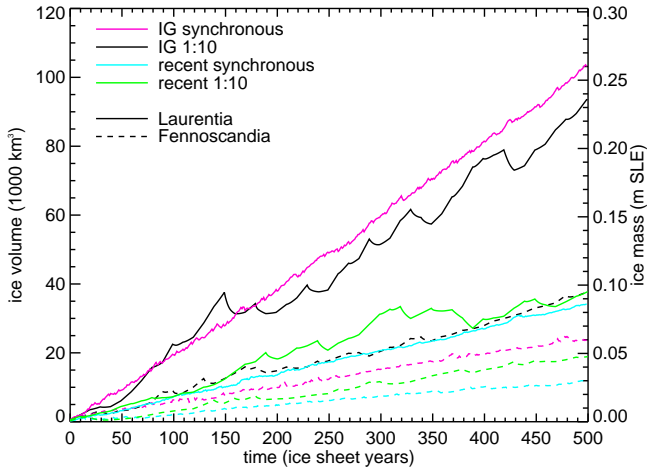
Fig. 3. Ice-sheet mass as a function of time for the first 500 years of the synchronous and asynchronous (1:10) experiments. Glimmer domains are indicated by linestyle, and experiments by colour. Values are annual means.
