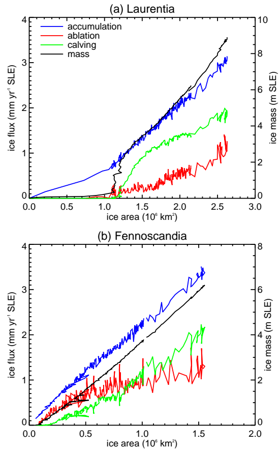
Fig. 14. Components of ice-sheet mass balance in the incipient glacial experiments integrated over the time-dependent ice-sheet area in each domain and shown as functions of that area. Values The first 25 ka of the timeseries are 100-year means for from the 1:10 experiment and , the remainder are 1000-year means for from the 1:100 experiment.
