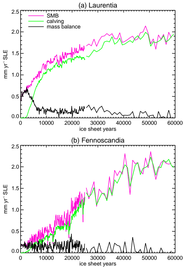
Fig. 13. Components of ice-sheet mass balance in the incipient glacial experiments shown as timeseries of area-integrals over the final ice-sheet area in each domain. Values The first 25 ka of the timeseries are 100-year means for from the 1:10 experiment and , the remainder are 1000-year means for from the 1:100 experiment.
