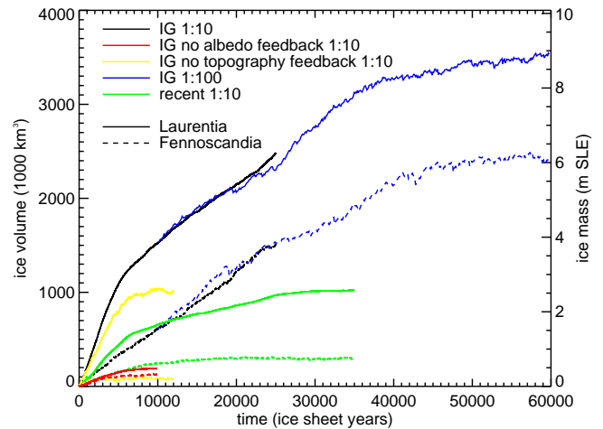
Fig. 5. Ice-sheet mass as a function of time through the whole length of the asynchronous (1:10 and 1:100) experiments. Glimmer domains are indicated by linestyle, and experiments by colour. Values are 100-year means.
