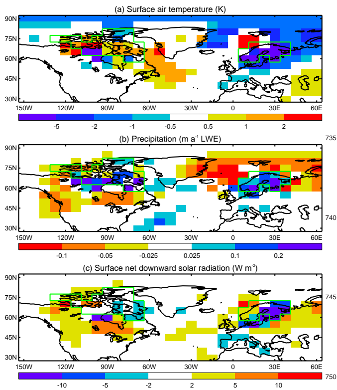
Fig. 10. Difference in the quantities indicated between the final steady state and the time-mean of years 1–100 of the synchronously coupled experiment for the incipient glacial climate (final minus initial). The green line shows the extent of the ice-sheet during years 1–100, as defined in the text. Changes are shown only where they differ from internal variability, as determined by a two-tailed Student t -test at a significance level of 5%.
