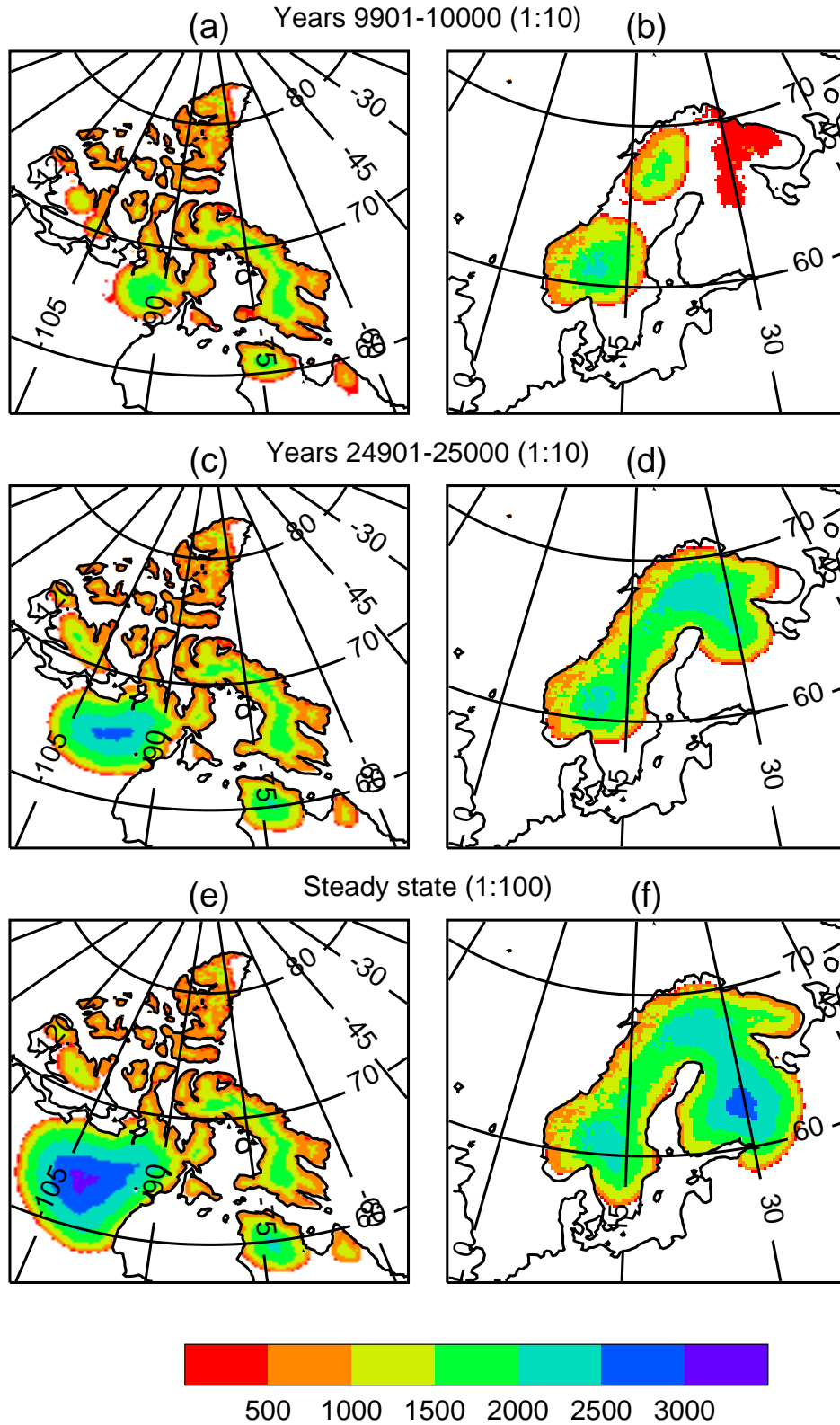
Fig. 8. Ice-sheet time-mean thickness (m) (a,b) after 10 ka, (c,d) after 25 ka and (e,f) in the steady state for the incipient glacial climate.
