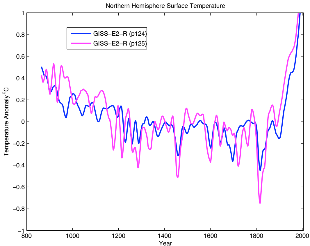
Fig. 1. NH surface air temperatures from GISS-E2-R (p124 and p125) (30yr smooth). Time-series uncorrected for control run drift. Note that the colours correspond to the correct labeling in Fig 9.
