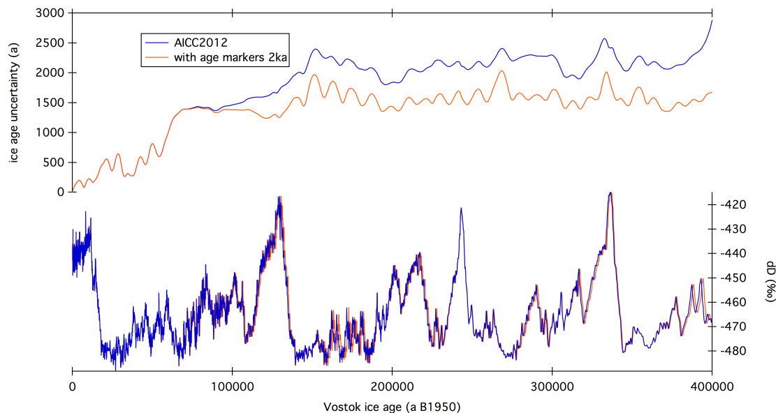
Fig. 2. Vostok chronology comparison of AICC2012 (blue) and Datice using 2ka uncertainty of \delta\text{O}_2/\text{N}_2 at Vostok (orange). Bottom: water isotope, top: ice age uncertainty calculated by Datice.
