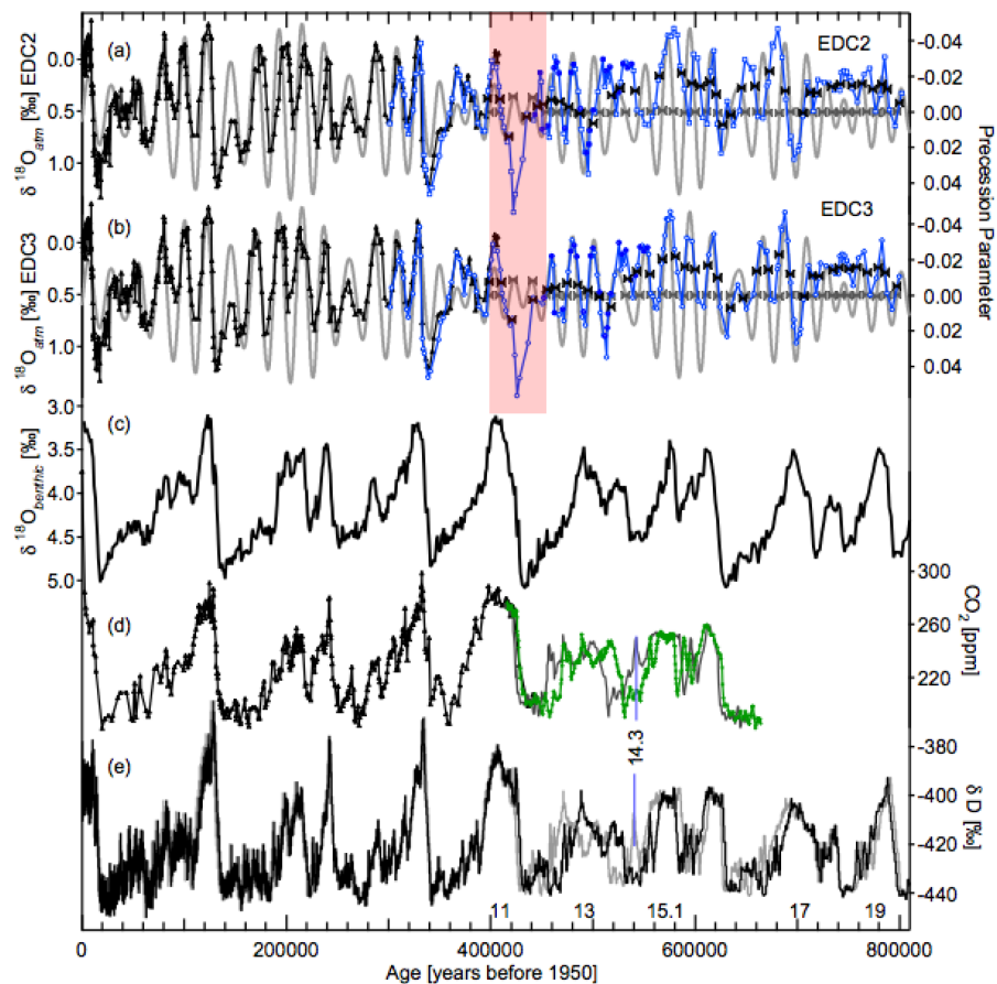
Fig. 5. Figure extracted from Dreyfus et al., 2007. The red box highlights the period where the orbital matching of \delta^{18}\text{O}_{\text{atm}} might be questionable.
