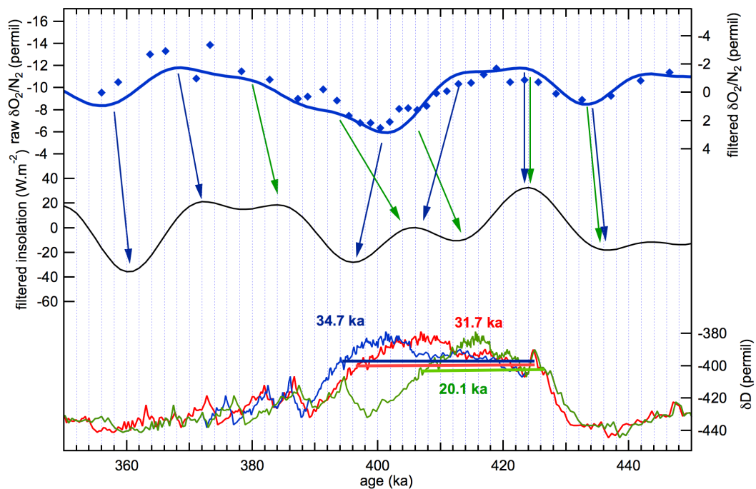
Fig. 4. Impact of \delta\text{O}_2/\text{N}_2 tuning on MIS 11 duration at EDC due to the lack of clear correspondence between \delta\text{O}_2/\text{N}_2 and local insolation curve.
