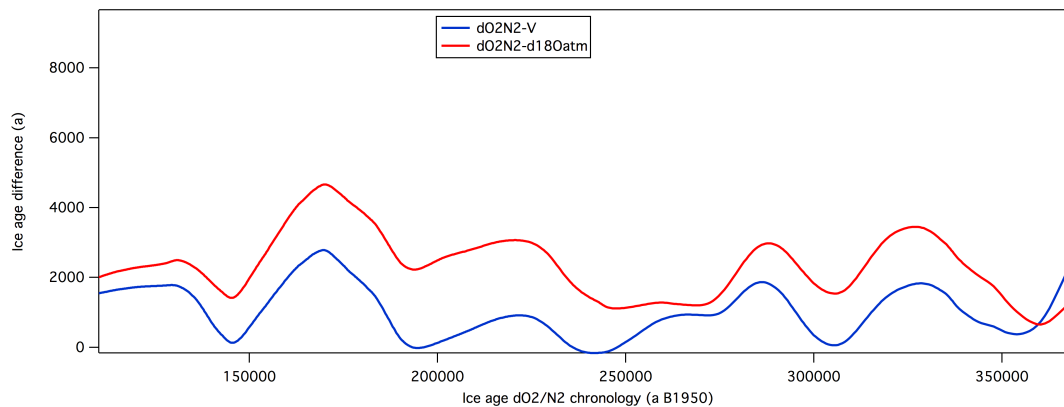
Fig. 3. Orbital chronology comparison in the case of a Vostok \delta\text{O}_2/\text{N}_2 age markers uncertainty of 2ka.
