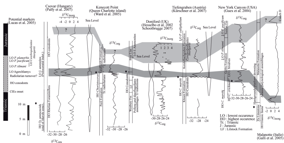
Fig. 1. Compilations of d13C data across the TJB
