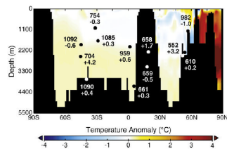
Figure 2: Modelled mean annual deep ocean temperature anomaly (Pliocene relative to modern) at 17°W (coloured background) and PRISM3D proxy-based bottom water temperature anomaly (Pliocene relative to modern) in the Atlantic Ocean (bullet points). From Robinson et al., 2011. Bathymetric controls on Pliocene North Atlantic and Arctic sea surface temperature and deepwater production. Palaeogeography, Palaeoclimatology, Palaeoecology , 309 (1-2), 92-97
