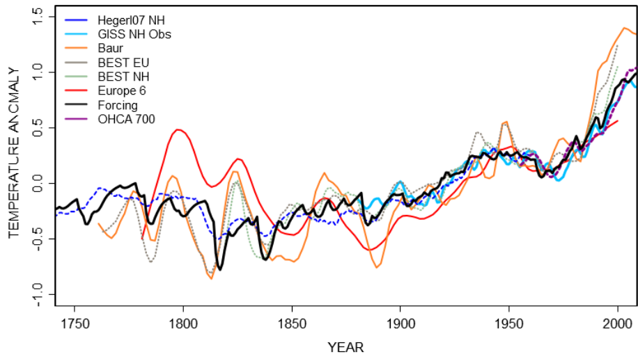
Europe 6 vs Instrumental Temperature vs Forcing Function
