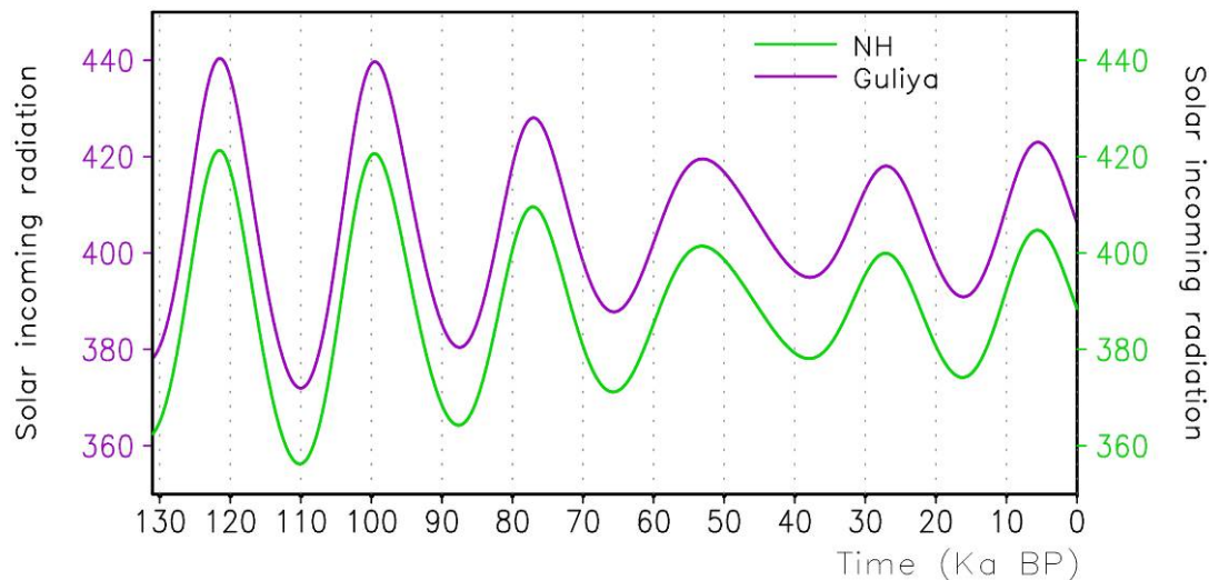
Fig. 4. Fig. D. Incoming solar radiation in the late summer over Guliya (Puple; left ordinate) and NH (Green; right ordinate) during the past 130 ka. The Unit is \text{W m}^{-2} .
