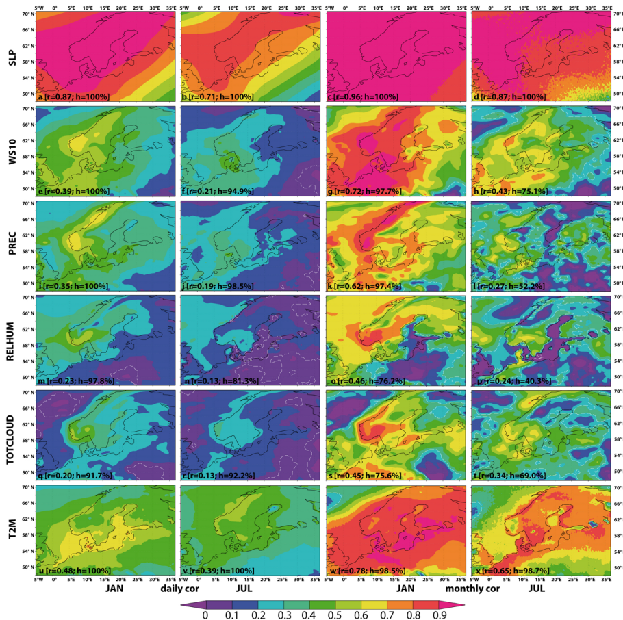
Fig. 6. Correlation maps on daily and monthly scale between HiResAFF and the reference fields of RCAO/ERA40 for January and July 1958–2007. White shaded lines indicate areas where h_0 of zero correlation cannot be rejected with p < 0.05 .
