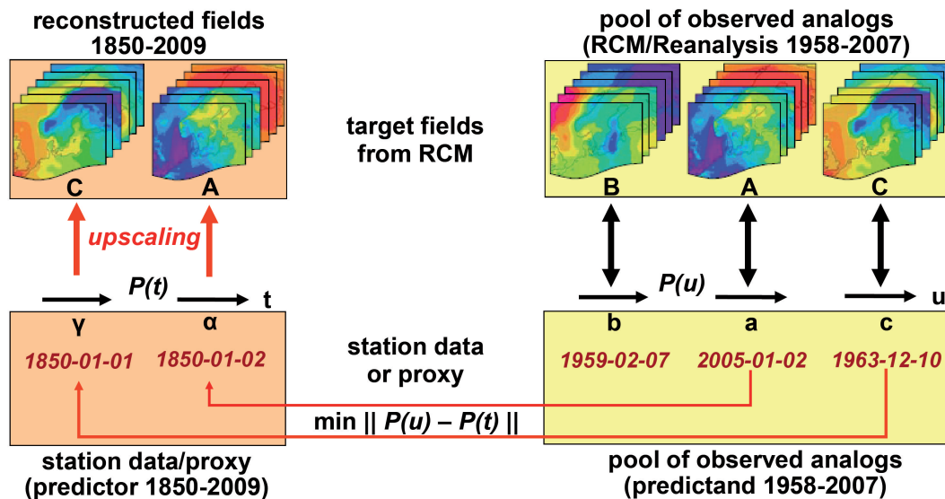
Fig. 1. Scheme for the Analog-Method used as upscaling tool. Any day a, b, c etc. of P(u) is linked to its related fields A, B, C etc. taken from RCM/Reanalysis (predictand, analogs). The fields of a historical day \gamma, \alpha etc. from P(t) is found by the Eq. (1) to be most similar to c, a etc. in P(u) forming the analog-pool. Hence, it is assumed, that the fields of \gamma, \alpha etc. are then very similar to the fields C, A etc. (upscaling).
