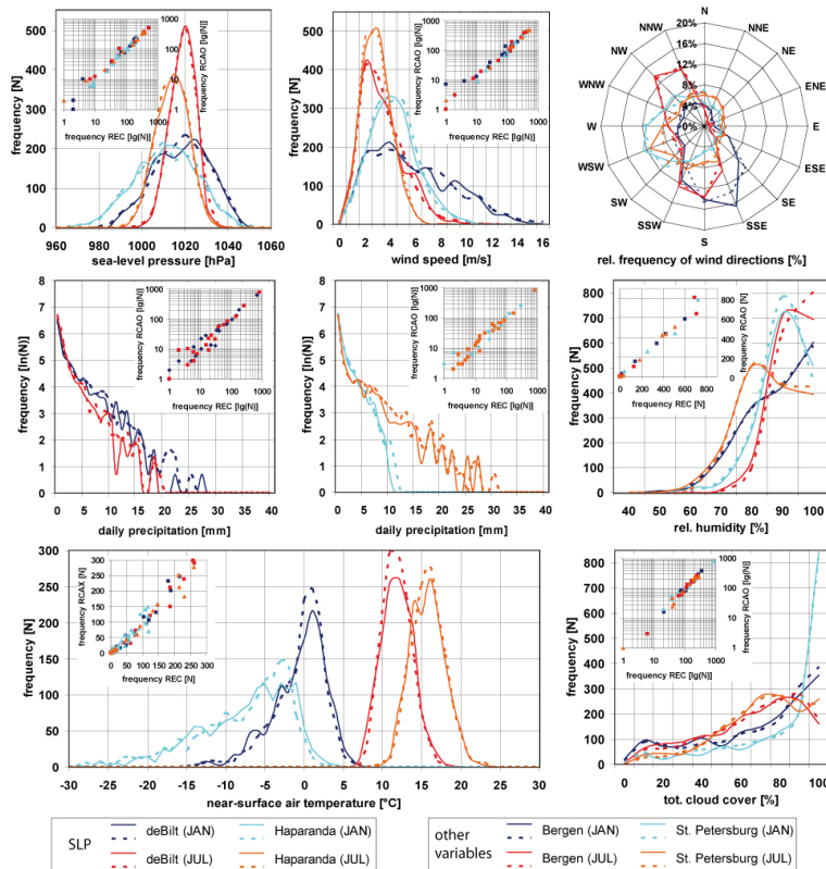
Fig. 9. Comparison of the frequency distributions between reconstruction (HiResAFF) and reference fields from RCAO (RCAX in case of temperature) for different variables. Grid points are chosen in the vicinity of de Bilt and Haparanda in case of SLP to highlight latitudinal changes. For other variables, Bergen and Saint Petersburg are chosen to depict differences between more maritime-advective (Bergen) and continental (Saint Petersburg) climate regimes. Embedded are the scatter plots of the regression between the reconstructed and simulated distributions. Note different usage of scaling (log, and ln).
