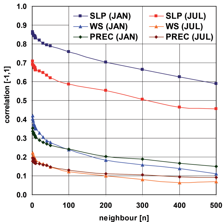
Fig. 4. Density of suitable analogs in HiResAFF estimated as the decay in daily correlation as a function of n next neighbours to the best analog chosen from around 4500 possible analogs. Displayed are the variables of SLP, wind speed (WS) and PREC for January and July.
