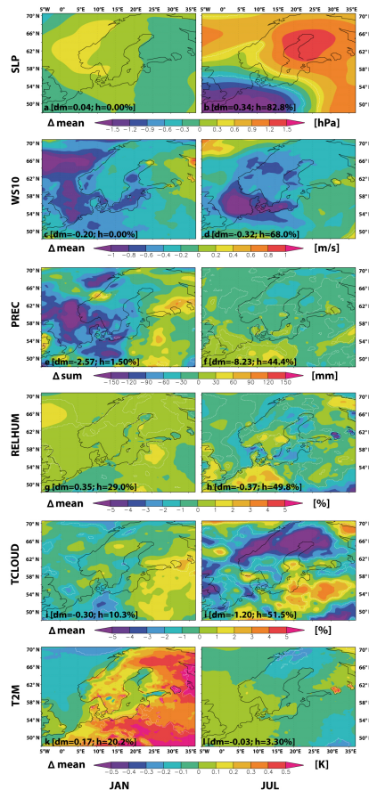
Fig. 8. Mean bias of HiResAFF minus the reference fields of RCAO/ERA40 for January and July 1958–2007. White shaded lines indicate areas where the reconstruction shows significant bias in mean with p < 0.05 .
