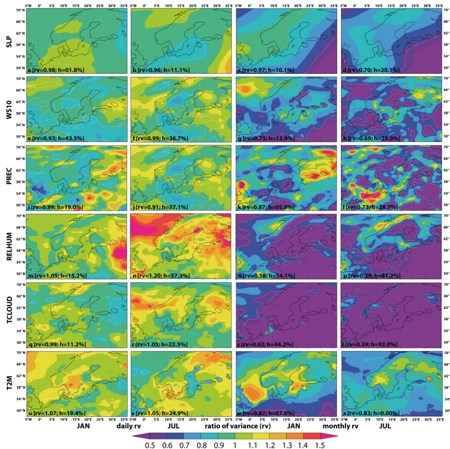
Fig. 7. Ratio of variance on daily and monthly scale between HiResAFF and the reference fields of RCAO/ERA40 for January and July 1958–2007. White shaded lines indicate areas where the reconstruction shows significant deviations in variance with p < 0.05 .
