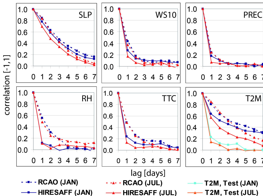
Fig. 10. Comparison of reconstructed daily auto-correlations of HiResAFF (solid lines) with the reference values derived from RCAO (shaded lines) for January and July at a grid point close to Stockholm. Additionally displayed test cases (light blue, orange) for T2M show the daily serial-correlation if T2M is reconstructed using the standard settings from Sect. 2.3.2.
