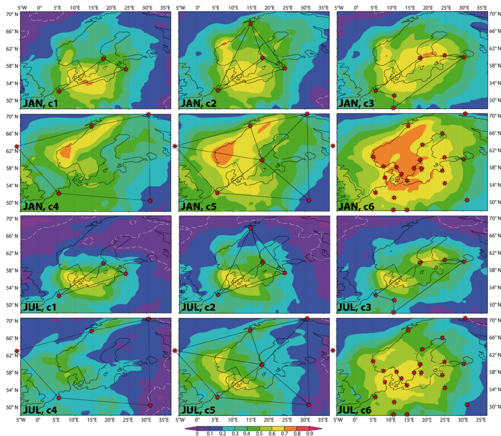
Fig. 5. Correlation of daily wind speeds between a surrogate reconstruction and reference fields of RCAO/ERA40 for January and July 1958–2007 dependent on the number and distribution of SLP predictors. White shaded lines indicate areas where h_0 of zero correlation cannot be rejected with p < 0.05 .
