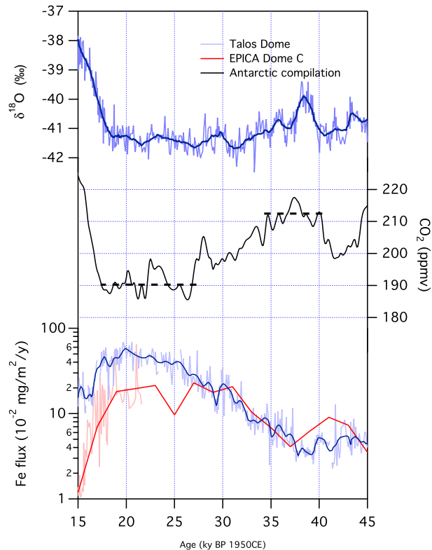
Fig. 4. Comparison of LGM Fe fluxes and late glacial drawdown of CO 2 . TALDICE δ 18 O paleotemperature values are from (Stenni et al., 2011). CO 2 concentrations were compiled from various Antarctic ice cores (Lüthi et al., 2008; Schilt et al., 2010) while Fe fluxes are shown for TD (this work) and EDC (Wolff et al., 2006; Gaspari et al., 2006) ice cores.
