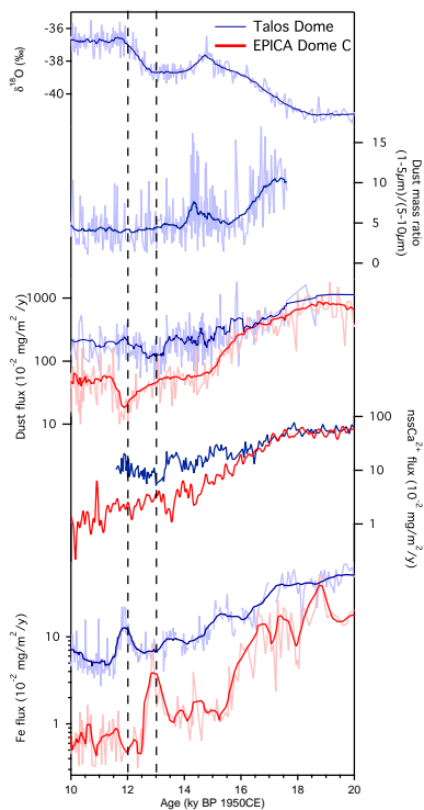
Fig. 2. Deglacial changes in Fe, nssCa 2+ and dust at Dome C and Talos Dome. TALDICE \delta^{18}\text{O} values are from (Stenni et al., 2011). Fine (1–5 \mu\text{m} )/coarse (5–10 \mu\text{m} ) dust particle ratios are from Albani et al. (2012) and dust fluxes are from Delmonte et al. (2010). nssCa 2+ data are shown for TD (this study) and EDC (Röthlisberger et al., 2004) ice cores. Deglacial EDC Fe fluxes are from Gaspari et al. (2006). The vertical dashed lines, located at 11.9 and 12.9 kyr BP, highlight enhanced Fe fluxes which occur independently of dust fluxes at Talos Dome and Dome C, respectively.
