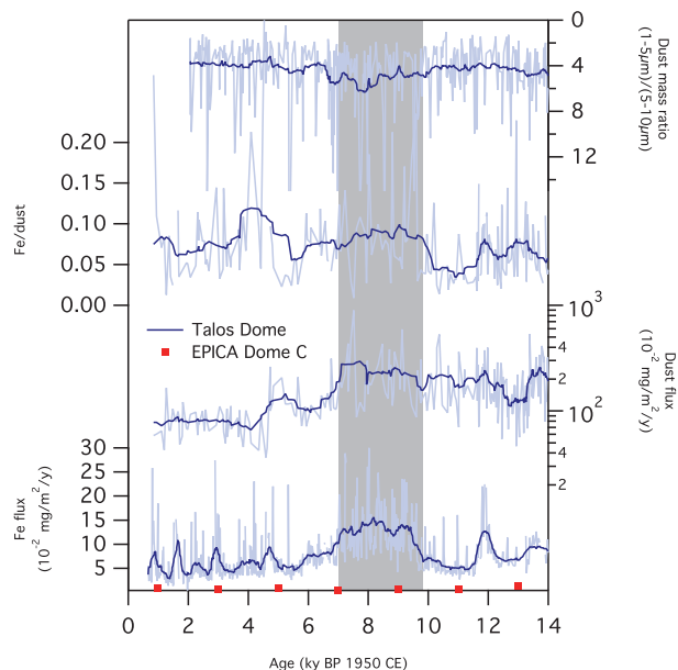
Fig. 3. Holocene Fe (this work) and dust (Delmonte et al., 2010) fluxes and fine (1–5 μm)/coarse (5–10 μm) dust particle ratios (Albani et al., 2012) in the TALDICE ice core (blue lines). EPICA Dome C dust fluxes (Wolff et al., 2006) are also shown (red squares). Note the fine/coarse dust particle ratios are plotted here on a reversed scale.
