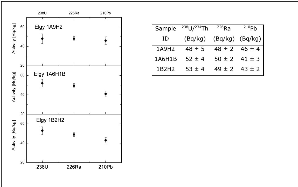
Figure S1: Activities of the U-series products for the three samples measured at VKTA Rossendorf. If the decay series is in equilibrium the activities of all daughters agree within 2-sigma errors with the activity of the mother. The error bars shown in the graphs represent the 1 sigma errors.
