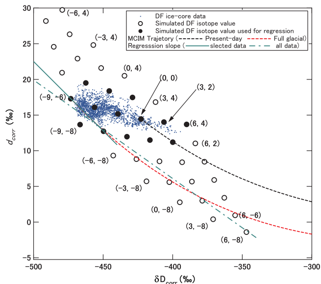
Fig. 4. Simulated \delta D and d values in Antarctica. Trajectories of present-day (black dotted line) and glacial conditions (red dotted line) are shown. Each point (solid or open circles) represents the simulated snow isotope values at DF site under a specific site and source temperature setting, shown as (\Delta T_{\text{site}}, \Delta T_{\text{source}}) in ^{\circ}\text{C} . The DF ice core data (blue dot), and data used for regression analysis were shown as black solid circle. Linear regression d/\delta D slopes of a constant \Delta T_{\text{source}} (= -6.0^{\circ}\text{C}) obtained for the filled circles and all circles are shown as green solid and chain lines, respectively. Here, \delta D and d are corrected for \delta^{18}\text{O}_{\text{sw}} , see text for detail.
