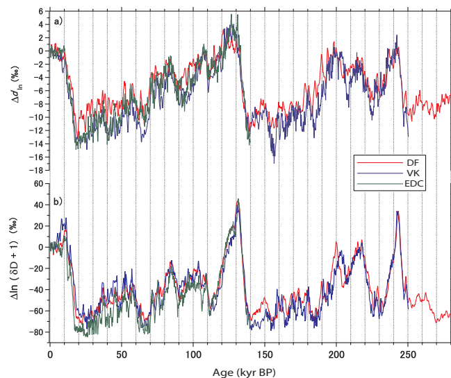
Figure A3. Logarithmic defined deuterium-excess and \delta D records of Antarctic ice cores. (a) Deuterium-excess based on logarithmic expression ( d_{in} ) records from DF (red line), Vostok (blue line), and EDC (green line) cores plotted on the O_2/N_2 orbital age scale for DF. (b) \ln(\delta D + 1) records of the three cores plotted on the O_2/N_2 orbital age scale for DF.
