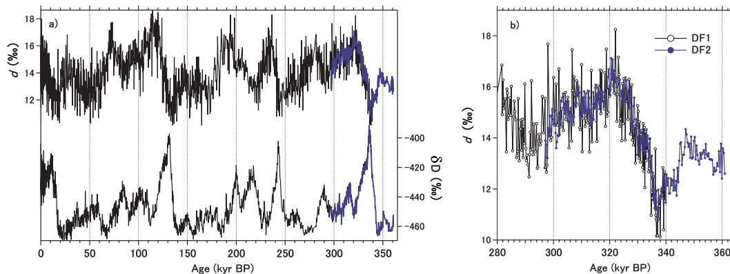
Fig. 1. \delta D and deuterium-excess records from the DF ice cores. (a) \delta D and d records from DF1 (black lines) and DF2 (blue lines) cores. (b) Enlarged view of the d records during the overlapping period. Here, \delta = R_{\text{sample}}/R_{\text{VSMOW}} - 1 , and R_{\text{sample}} and R_{\text{VSMOW}} are the isotope ratios ( D/H and ^{18}\text{O}/^{16}\text{O} ) of sample and VSMOW, respectively.
