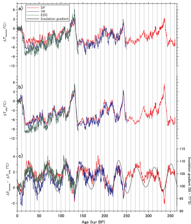
Fig. 6. The \Delta T_{\text{site}} , \Delta T_{\text{source}} , and the temperature gradient derived from the three cores. Temperature records reconstructed from the DF (red line), Vostok (blue line), and EDC (green line) cores using the isotope-fitting method. (a) \Delta T_{\text{source}} , (b) \Delta T_{\text{site}} , (c) Temperature gradient ( = \Delta T_{\text{source}} - \Delta T_{\text{site}} ) and annual mean insolation gradient between 50 and 77° S ( \text{W m}^{-2} , black dotted line).
