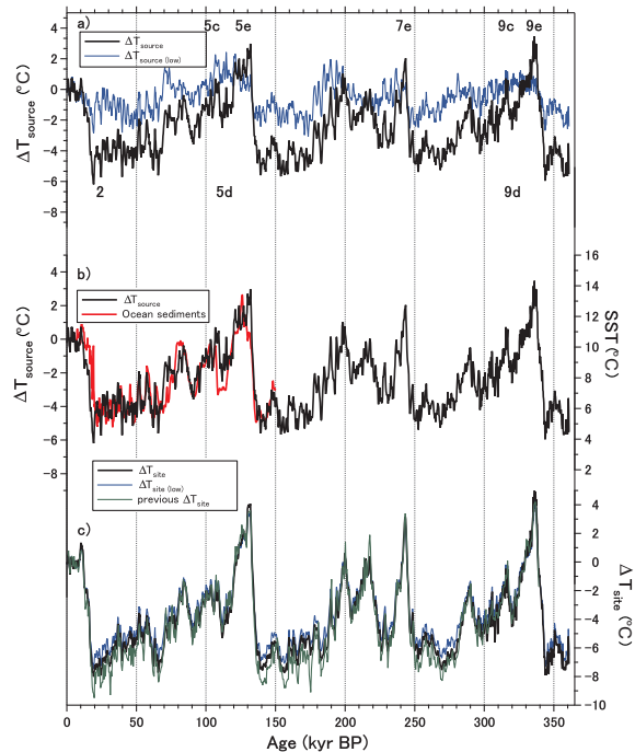
Fig. 5. Different \Delta T_{\text{source}} and \Delta T_{\text{site}} of DF and a stacked SST records. (a) Black line represents the \Delta T_{\text{source}} record of DF core based on the coefficients ( \beta_{\text{site}} = 1.3 ) obtained by isotope-fitting (this study). Blue line represents the \Delta T_{\text{source}}^{\text{low}} record of DF core based on the coefficients ( \beta_{\text{site}} = 0.5 ) used for Vostok reconstruction (temperature-fitting) (Cuffey and Vimeux, 2001; Vimeux et al., 2002). Numbers indicate Marine Isotope Stages. (b) Black line is the \Delta T_{\text{source}} of DF core, same as (a) , but with a stacked southern SST record of ocean sediments (Barrows et al., 2007) (red line). (c) The \Delta T_{\text{site}} record based on the coefficients of this study (black line), \Delta T_{\text{site}}^{\text{low}} (blue line), and previous \Delta T_{\text{site}} reconstruction of DF core (temperature-fitting) (Kawamura et al., 2007).
