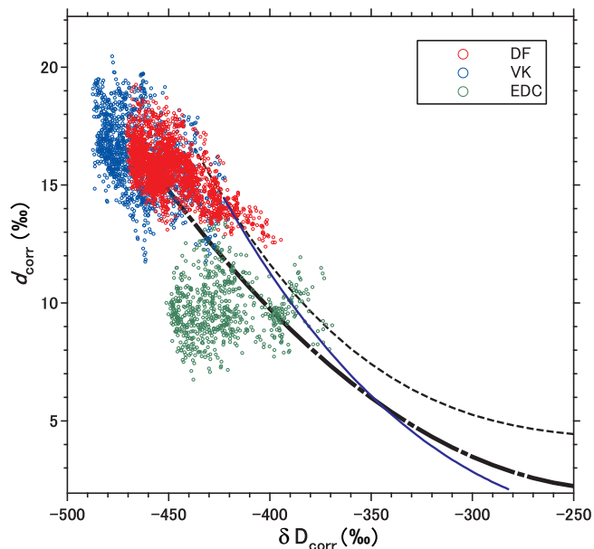
Fig. 3. Isotope ratios of Antarctic surface snow and ice cores. Regression curves of surface snow data from various parts of Antarctica (black dashed-dotted line) (Masson-Delmotte et al., 2008), and from Japanese-Swedish IPY 2007/2008 traverse covering Syowa-Dome F route (black dotted line). A simulated curve is shown as blue solid line. Dots represent ice-core data of DF over the past 360 kyr (red), Vostok over the past 250 kyr (blue), and EDC over the past 140 kyr (green). Here, \delta D and d are corrected for \delta^{18}O_{sw} , see text for detail.
