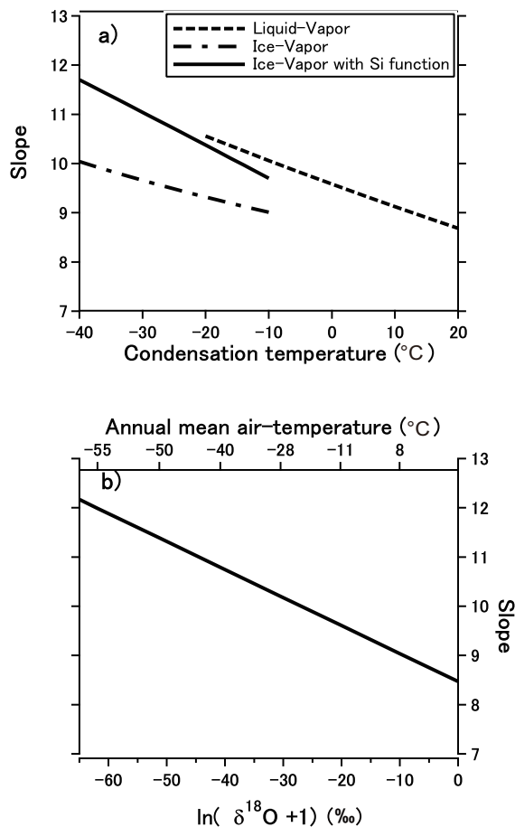
Figure A2. Slopes based on fractionation factors and GMWC. The \delta D/\delta^{18}O slope is calculated using a differential of Eq. (7) ( = -5.70 \times 10^{-2} \times \ln(1 + \delta^{18}O) + 8.47 ). Kinetic fractionation during snow formation was considered using a super-saturation function (see text).
