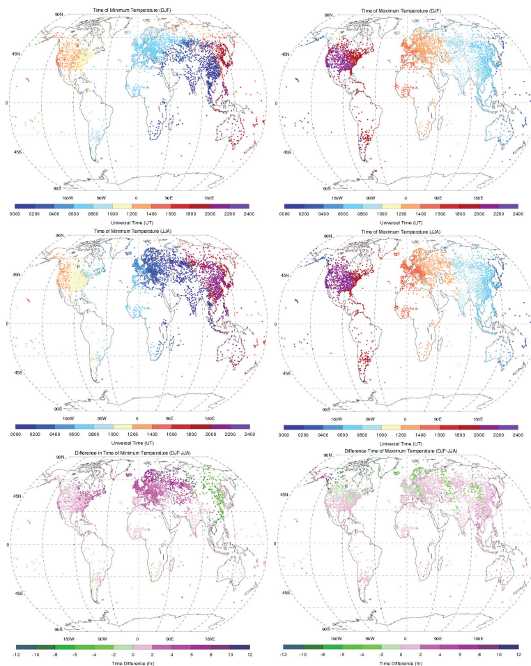
Fig. 21. The median times of the minimum (left) and maximum (right) temperature recorded by each station (using the selected 3375 stations). Top for December-January-February, Middle for June-July-August. Bottom shows the difference in the times between DJF and JJA for the minimum and maximum temperatures.
