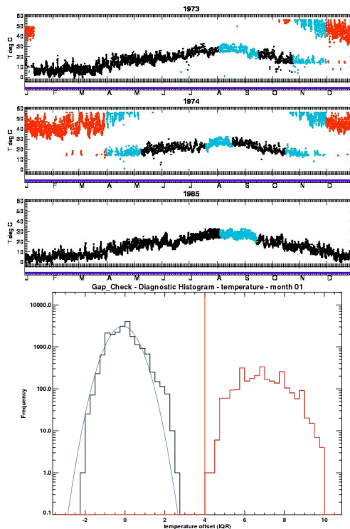
Fig. 7. Top: distributional gap check (test 6) example when comparing all of a given calendar month in the dataset for station 476960-43323, Yokosuka, Japan ( 35.58^{\circ} N, 139.667^{\circ} E, 530 m), an assigned composite station, showing temperature for the years 1973, 1974 and 1985. Red points show values removed by this test and blue points by other tests (in this case, mainly the diurnal cycle check). There is no change in source station in any of the years, and so compositing has not caused the bad data quality of this station. Bottom: distribution of the observations from all Januaries in the station record. The population highlighted in red is removed by this test. Note logarithmic y-axis.
