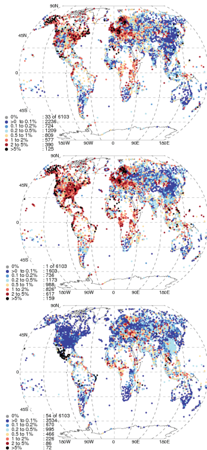
Fig. 19. Rejection rates by variable for each station. Top panel: T, middle panel: Td and lower panel: SLP. Different rejection rates are shown by different colours and the inline key in each panel provides total number of stations in each band.
