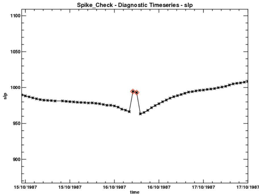
Fig. 15. The sea level pressure data from station 032450-99999 (Newcastle WX Centre, 54.967° N, -1.617° W, 47 m) on the night of the 16 October 1987. The two observations which have triggered the spike check are clearly visible and are distinct from the rest of the data. Given their values (994.6 and 993.1 hPa), the two flagged observations are clearly separate from their adjacent ones (966.4 and 963.3 hPa) it is possible that a keying error in the SYNOP report lead to 946 and 931 being reported, rather than 646 and 631. However, we make no attempt in this dataset to rescue flagged values.
