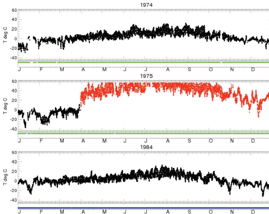
Fig. 6. Distributional gap check (test 6) example for station 714740-99999, Clinton, BC, Canada ( 51.15^{\circ}\text{N} , 121.50^{\circ}\text{W} , 1057 m), an assigned composite station, showing temperature for the years 1974, 1975 and 1984. Red points show values removed by this test and blue points by other tests. The panel below each year shows whether the data in the composited station come from the named station (purple) or a matched station (green). There is no change in source station within 1975, and so the compositing has not caused the clear offset observed therein, but the source station has changed for 1984 compared to the other two years.
