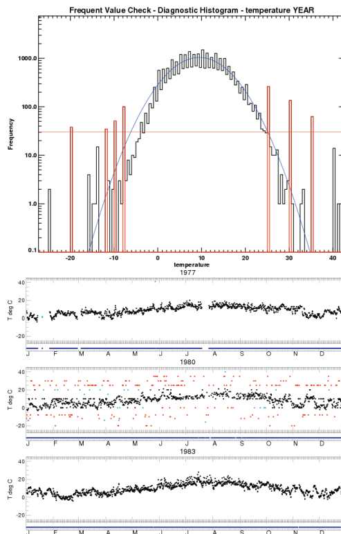
Fig. 4. Frequent value check (test 4) for station 037930-99999, Anvil Green, Kent, UK ( 51.22^{\circ} N, 1.000^{\circ} E, 140 m) showing temperature. Top panel: histogram (note logarithmic y-axis) for entire station record showing the bins which have been identified as being likely frequent values. Bottom panel: red points show values removed by this test and blue points by other tests for the years 1977, 1980 and 1983. The panel below each year indicates which station the observations come from in the case of a composite (not relevant here but is relevant in other station plots so included in all).
