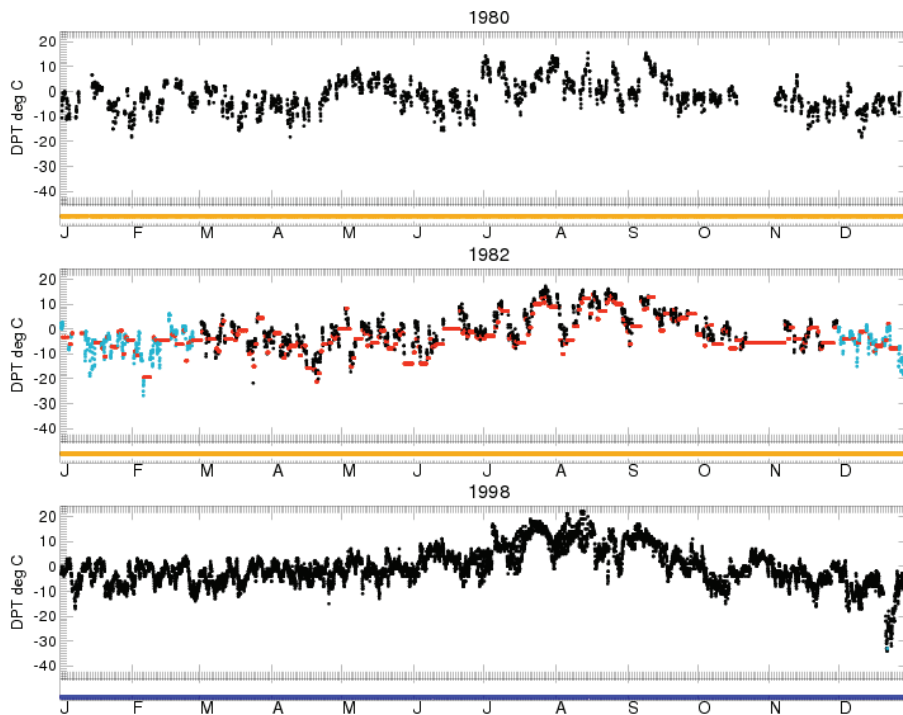
Fig. 8. Repeated streaks/unusual streak frequency check (test 8) example for station 724797-23176 (Milford, UT, USA 38.44^{\circ}\text{N} , 112.038^{\circ}\text{W} , 1534 m), an assigned composite station, for Dewpoint temperature in 1982, illustrating frequent short streaks. Red points show values removed by this test and blue points by other tests. The panel below each year shows whether the data in the composited station come from the named station (blue) or a matched station (orange). There is no change in source station in 1982, and so the compositing has not caused the streaks observed in 1982, but a different station is used in 1998 compared to the other two years.
