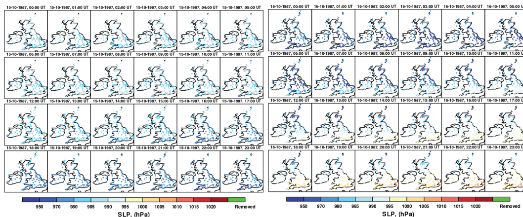
Fig. 14. Passage of low pressure core over the British Isles during the night of 15 and 16 October 1987. Green points (highlighted by circles) are stations where the observation for that hour has been removed. There are two, at 05:00 and 06:00 UTC on 16 October 1987 in the north-west of England. The station which has these two flagged observations is shown in Fig. 15.
