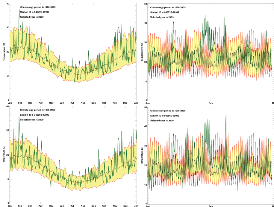
Fig. 18. Left: daily mean temperature in Southern Australia in 2009 (green curve) with climatological average (black line) and 5th and 95th percentiles (red lines and yellow shading). The exceptionally high temperatures in late January/early February and mid-November can clearly be seen. Right: similar plots showing the full synoptic resolution for a two month period starting in January 2009. The climatology, 5th and 95th percentile lines have been smoothed using an 11-point binomial filter in all four plots. Top: Adelaide (946725-99999, 34.93° S, 138.53° E, 4 m), bottom: Melbourne (948660-99999, 37.67° S, 144.85° E, 119 m).
