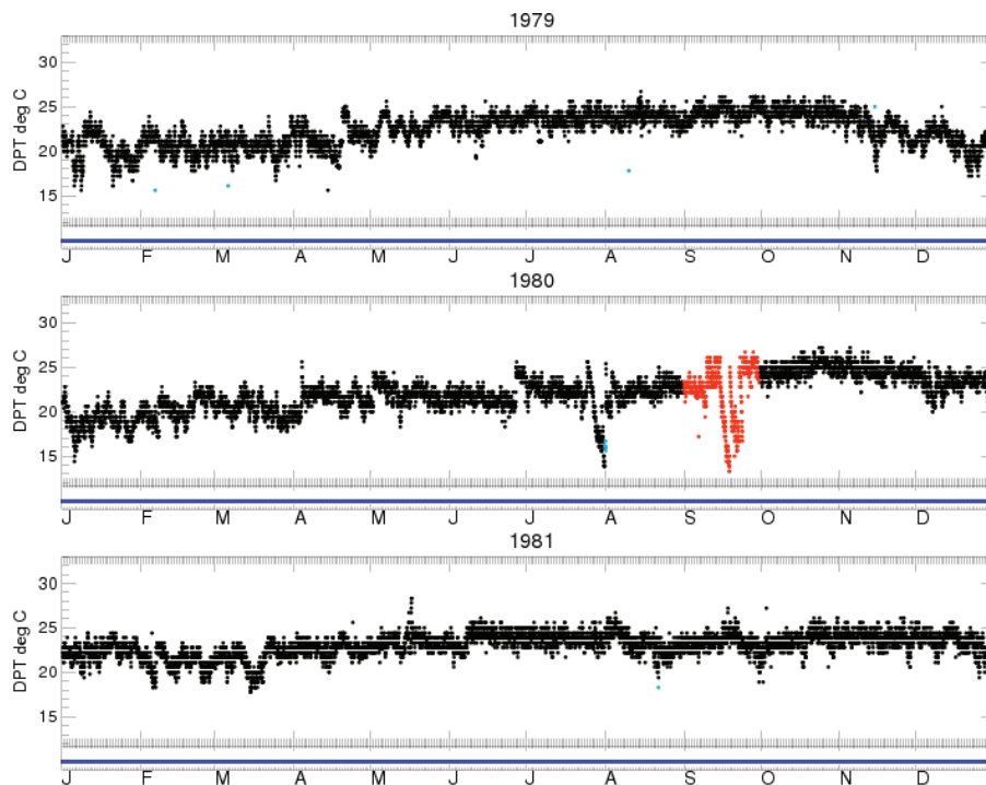
Fig. 12. Unusual variance check (test 13) for station 912180–99999 (13.57° N, 144.917° E, 162 m, Anderson Airforce Base, Guam) for dewpoint temperature. Red points show values removed by this test and blue points by other tests.
