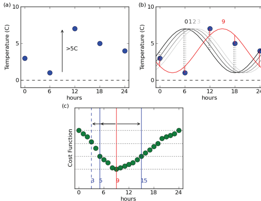
Fig. 5. Schematic for the diurnal cycle check. (a) An example timeseries for a given day. There are observations in more than 3 quartiles of the day and the diurnal range is more than 5^{\circ}\text{C} so the test will run. (b) A sine-curve is fitted to the days observations. In this schematic case, the best fit occurs for a 9 h shift. The cost function used to calculate the best fit is indicated by the dotted vertical lines. (c) The cost function distribution for each of the possible 24 offsets of the sine curve for this day. The terciles of the distribution are shown with the horizontal black dotted lines. Where the cost function values cross into the second tercile, determines the uncertainty (vertical blue lines). The larger of the two differences (in this case 9\ 15 = 6\text{ h} ) is chosen as the uncertainty. Therefore if the climatological value is between 3 and 15 h, then this day does not have an anomalous diurnal cycle phase.
