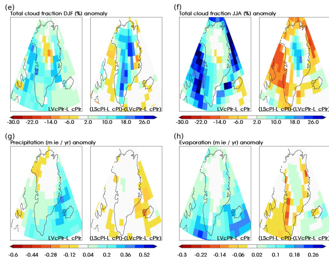
Fig. 4. (e) as (a), but for boreal winter mean total cloud cover. (f) as (a), but for boreal summer mean total cloud cover. (g) as (a), but for annual mean precipitation (m i.e. \text{yr}^{-1} ). (h) as (a), but for annual mean evaporation (m i.e. \text{yr}^{-1} ).
