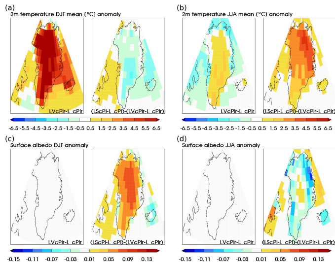
Fig. 4. (a) Climatological mean boreal winter (DJF) 2 m-temperature, difference between simulations with modified vertical levels and the standard version (LVcPIr – L_cPIr, left) and difference from introducing the snow scheme (LScPI – L_cPI – LVcPIr + L_cPIr, right). (b) as (a), but for boreal summer (JJA). (c) as (a), but for boreal winter mean surface albedo. (d) as (a), but for boreal summer mean surface albedo.
