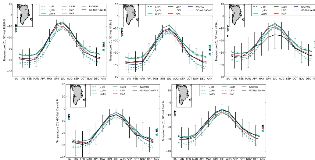
Fig. A1. Climatological monthly mean 2 m-temperature ( ^{\circ}\text{C} ) in Greenland as in Fig. 1, but at the GC-net AWS stations (Steffen et al., 1996) TUNU-N, NASA-E, NASA-U, Crawford Point, SADDLE, compared to interpolated model data. Vertical bars show interannual standard deviation for the observation data; triangles indicate the seasonal mean for boreal summer (left) and the annual mean (right).
