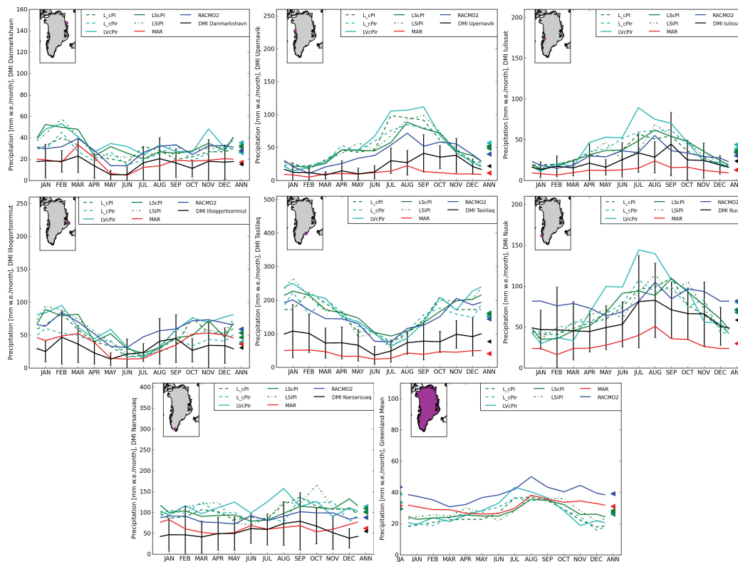
Fig. A2. As first part of Fig. A2, but at the DMI weather stations Danmarkshavn, Upernavik, Ilulissat, Iloqqortoormiut, Tasiilaq, Nuuk, and Narsarsuaq. Also shown is the comparison of the mean model precipitation for all of Greenland.
