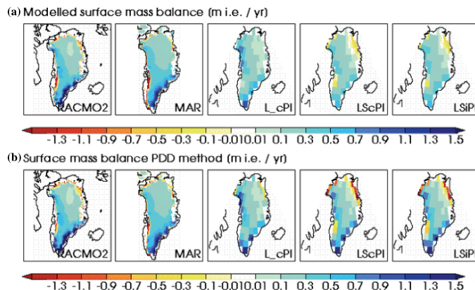
Fig. 3. (a) Climatological annual mean surface mass balance modelled on Greenland, from left to right for the regional models RACMO and MAR, the LMDZ reference simulation and LMDZ-SISVAT with constant climatological and variable lower boundary conditions. (b) as (a), but for SMB computed with the PDD method (m i.e. yr -1 ).
