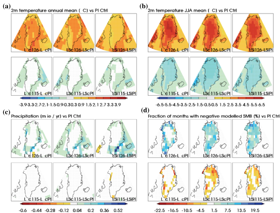
Fig. 6. (a) Climatological annual mean 2 m-temperature anomaly vs. preindustrial simulation (°C) in Greenland for Eemian (top row) and glacial inception (bottom row) simulations, in standard LMDZ (left) and LMDZ-SISVAT with constant climatological (center) and varying (right) lower boundary conditions. (b) as (a), but for climatological mean boreal summer (JJA) temperature (°C). (c) as (a), but for climatological annual mean precipitation (m i.e. yr -1 ). (d) as (a), but for annual mean fraction of months with negative modelled surface mass balance.
