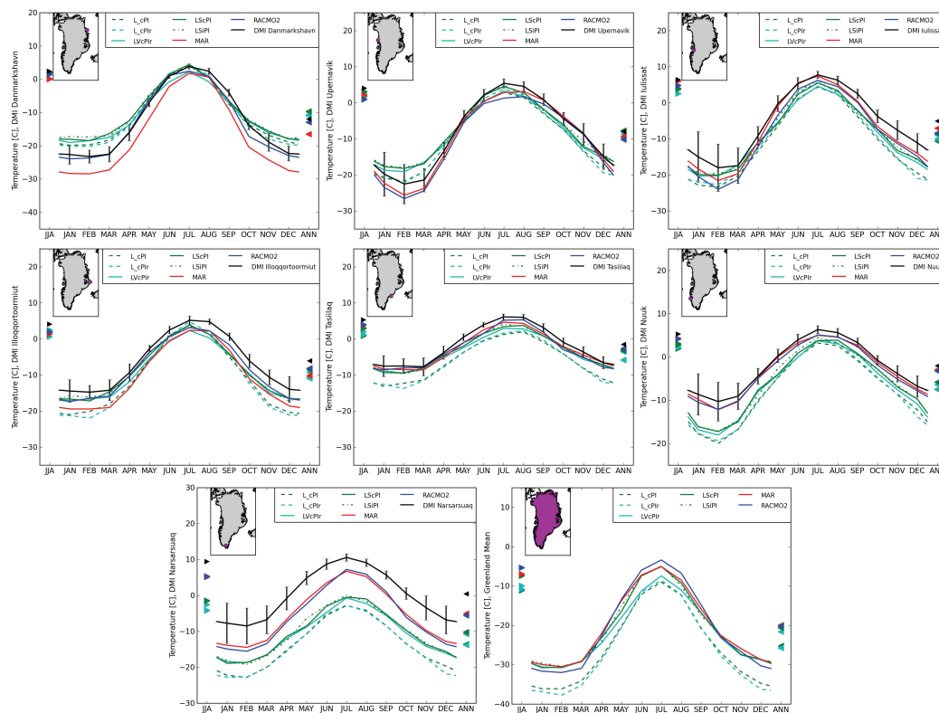
Fig. A1. As first part of Fig. A1, but for the DMI weather stations at Danmarkshavn, Upernavik, Ilulissat, Illoqqortoormiut, Tasiilaq, Nuuk and Narsarsuaq. Also shown is the comparison of the mean model temperature for all of Greenland.
