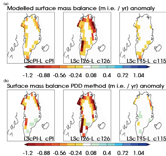
Fig. 5. (a) Climatological annual mean modelled SMB anomaly ( \text{m i.e. yr}^{-1} ) LMDZ-SISVAT – standard LMDZ in Greenland ( ^{\circ}\text{C} ) for preindustrial (left), Eemian (center) and glacial inception (right) simulations. (b) as (a), but for SMB computed with the PDD method ( \text{m i.e. yr}^{-1} ).
