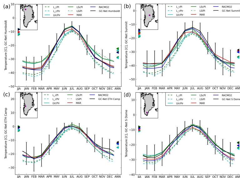
Fig. 1. Climatological monthly mean 2 m-temperature ( ^{\circ}\text{C} ) in Greenland at selected AWS stations of the GC-net (Steffen et al., 1996), compared to interpolated model data. (a) Humboldt, (b) Summit, (c) ETH-Camp, (d) South Dome. Vertical bars show interannual standard deviation for the observation data; triangles indicate the seasonal mean for boreal summer (left) and the annual mean (right).
