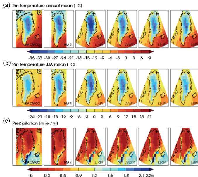
Fig. 2. (a) Climatological annual mean 2 m-temperature (°C) in Greenland, from left to right for the regional models RACMO and MAR, the LMDZ reference simulation (L c PI), LMDZ with modified levels (LV c PI), and LMDZ-SISVAT with constant climatological and variable IPSL-CM4 lower boundary conditions (LScPI and LSiPI). (b) as (a), but for climatological June-July-August seasonal mean 2 m-temperature (°C). (c) as (a), but for climatological annual mean precipitation (m i.e. yr -1 ).
