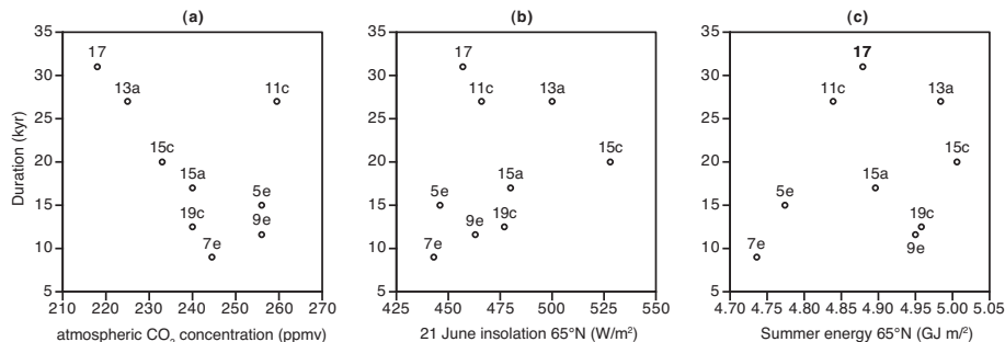
Fig. 10. Plot of atmospheric CO 2 and boreal summer insolation values at the time of glacial inception versus interglacial duration. (a) CO 2 concentration at inception versus duration; (b) summer insolation intensity (21 June insolation) at 65° N (Laskar et al., 2004) versus interglacial duration; (c) summer insolation energy at 65° N, defined as the sum of the diurnal average insolation on days exceeding 275 W m -2 (Huybers, 2006) versus interglacial duration.
