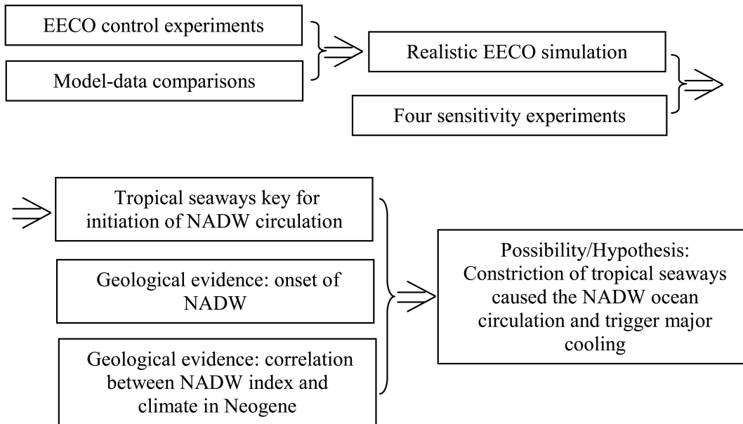
Fig. 1. Figure 1. Logical arguments for the paper
