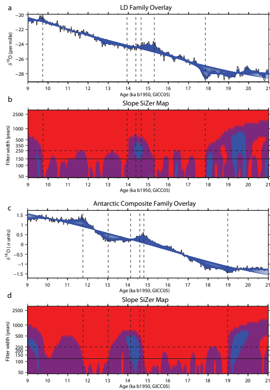
Fig. 1. Fig. 3. 'SiZer maps' of the significance of features in LD \delta^{18}O and the Antarctic composite through the deglaciation (see manuscript for full caption).
