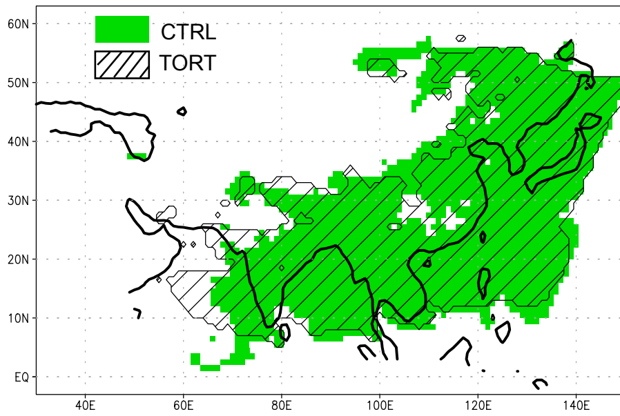
Fig. 1. Distribution of monsoonal climate in CTRL and TORT based on the method described by Wang & LinHo (2002).
