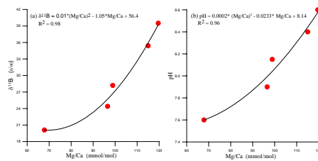
Fig. 9 Relationship (a) between Mg/Ca and \delta^{11}\text{B} in inorganic calcite, and (b) between Mg/Ca and seawater pH (Xiao et al., 2006a). The Mg/Ca was positive with \delta^{11}\text{B} in inorganic calcite and increased with seawater pH, which provide a new method for differentiating the existence of brucite in corals.
