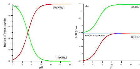
Fig. 1. Fraction (a) of the major dissolved boron species B(OH)_3 (green curve) and B(OH)_4^- (red curve) in seawater, using pK_a=8.597 (Dickson, 1990) and stable boron isotope fractionation (b) between them as a function of pH, using \alpha_{34}=0.974 (Klochko et al., 2006). At low pH (pH<7), virtually all of the boron in seawater is in the B(OH)_3 species; conversely, at high pH (pH>10), virtually all of the boron is in the B(OH)_4^- species (Fig. 1a). Only the B(OH)_4^- incorporated into the marine bio-carbonates is one of the essential hypotheses for using boron isotopic composition in marine bio-carbonate to reconstruct the paleo-environment (Hemming and Hanson, 1992).
