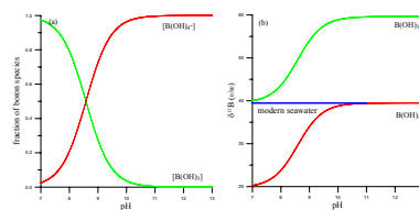
Fig. 1. Fraction (a) of the major dissolved boron species \text{B}(\text{OH})_3 (green curve) and \text{B}(\text{OH})_4^- (red curve) in seawater, using pK_a=8.597 (Dickson, 1990) and stable boron isotope fractionation (b) between them as a function of pH, using \alpha_{\text{B}}=0.974 (Kishchko et al., 2006). At low pH (pH<7), virtually all of the boron in seawater is in the \text{B}(\text{OH})_3 species; conversely, at high pH (pH>10), virtually all of the boron is in the \text{B}(\text{OH})_4^- species (Fig. 1a). Only the \text{B}(\text{OH})_3 incorporated into the marine bio-carbonates is one of the essential hypotheses for using boron isotopic composition in marine bio-carbonate to reconstruct the paleo-environment (Hemming and Hanson, 1992).
