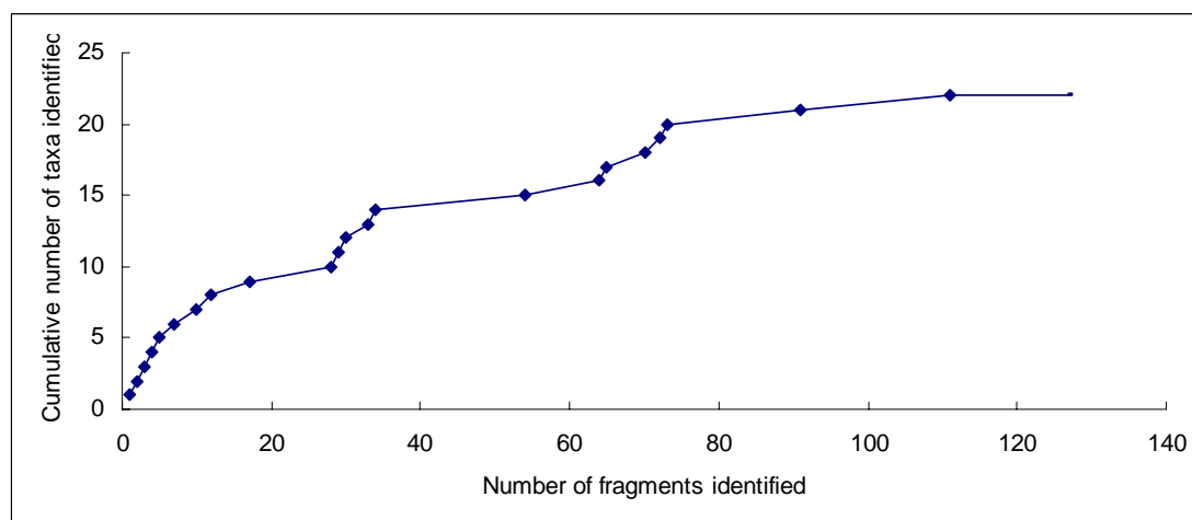
Identification saturation curve from the Dadiwan site, China.
