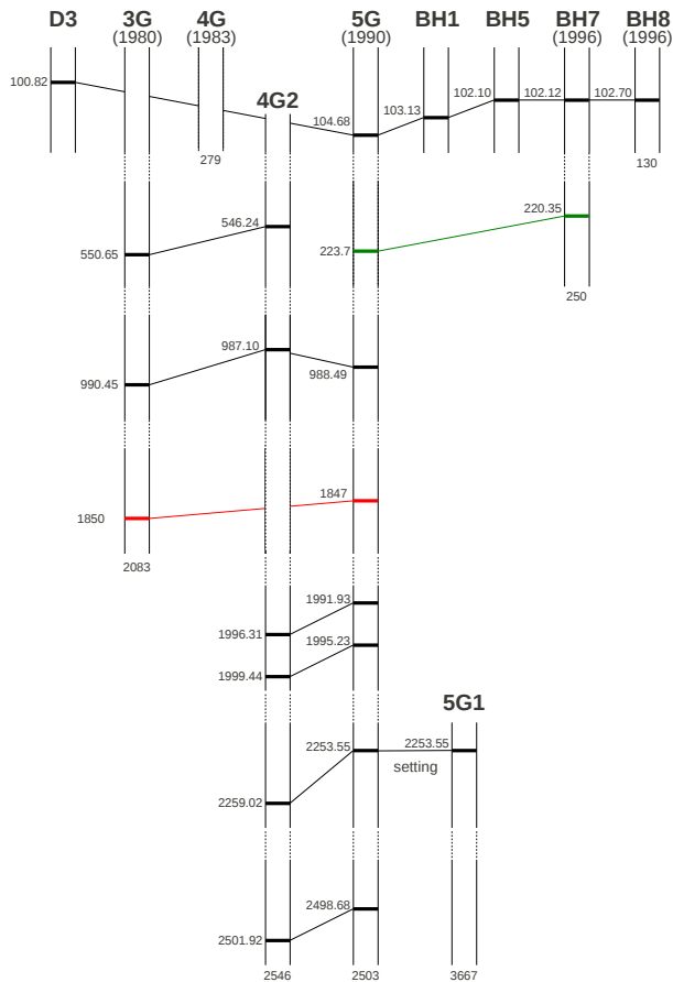
Fig. 3. Scheme of the different Vostok cores and shifts between them based on tephra recognition (black), ice isotopes synchronisation (red) and ECM synchronisation (green).
