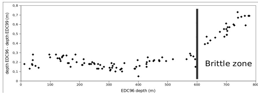
Fig. 4. Volcanic synchronisation of the EDC96 and EDC99 ice cores using the DEP records. (A) DEP records and volcanic tie points. (B) Resulting depth offset between EDC96 and EDC99. The vertical bar marks the start of the brittle zone.
