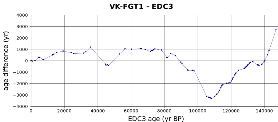
Fig. 10. Comparison of the VK-FGT1 and EDC3 time scales at the volcanic synchronisation tie points.
