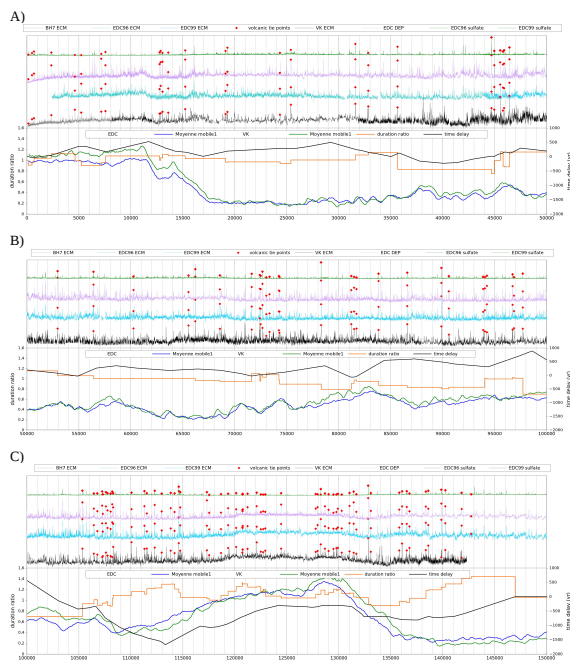
Fig. 7. EDC/VK volcanic synchronisation on the EDC3 age scale. (A) 0–50 kyr BP; (B) 50–100 kyr BP; (C) 100–150 kyr BP For (A) , (B) , (C) : Top Black: ECM record from the VK-5G ice core. Grey: ECM record from the VK-BH7 ice core. Blue: ECM record from the EDC99 ice core. Pink: DEP record from the EDC99 ice core. Green: sulfate records from the EDC96 and EDC99 ice cores. Red diamonds: volcanic tie points. Bottom Blue: Deuterium record from the EDC ice core. Green: Deuterium record from the Vostok ice core. The deuterium records have been resampled every 50 yr and an 11 points moving average was applied. Orange: ratio of the duration between two tie points in VK-FGT1 (Parrenin et al., 2004) and EDC3 (Parrenin et al., 2007b). Black: time delay between the VK-3G and EDC deuterium records after volcanic synchronisation.
