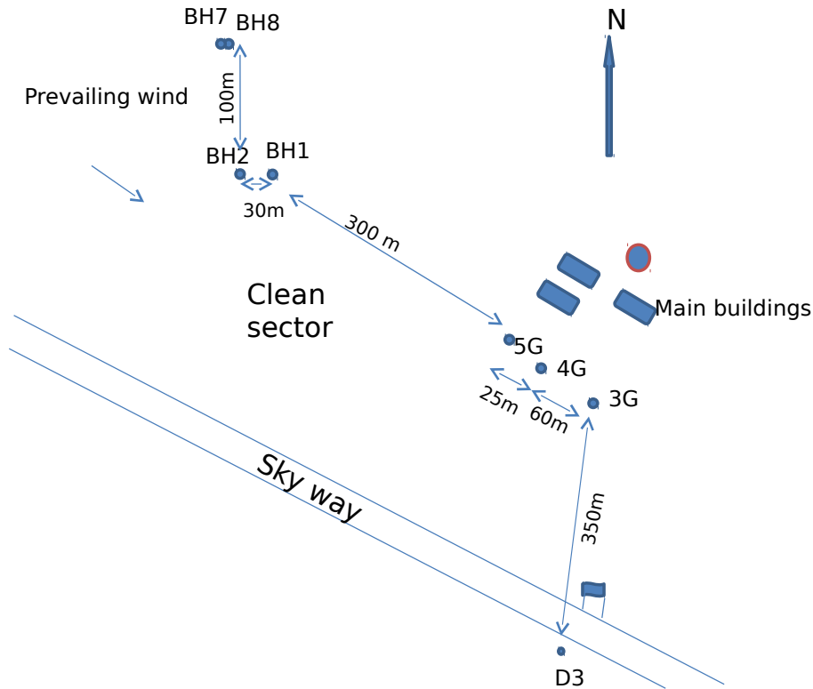
Fig. 2. Map illustrating the location of the camp facilities as well as the different boreholes considered in this study at Vostok station.
