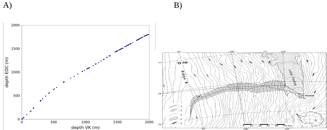
Fig. 9. (A) Volcanic tie points in a depth-VK/depth-EDC diagram. (B) The flow line between Ridge B and Vostok. Adapted from Salamatin et al. (2009). The steep slope in graph (A) between 0 and 500 m in VK corresponds to the lake part of the flow line, where the accumulation and berock elevation are lower than upstream.
