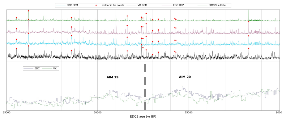
Fig. 11. Synchronisation during the period 65–80 kyr BP including the Toba eruptive event on the EDC3 age scale. Top Black: ECM record from the VK-5G ice core. Blue: ECM record from the EDC99 ice core. Pink: DEP record from the EDC99 ice core. Green: sulfate records from the EDC96 and EDC99 ice cores. Red diamonds: volcanic tie points. Bottom Blue: Deuterium record from the EDC ice core. Green: Deuterium record from the Vostok ice core.
