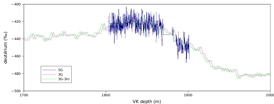
Fig. 6. Vostok ice isotopic composition during termination II, for the 3G and 5G ice cores. A depth shift of several meters (typically 3 m) between both cores is likely.
