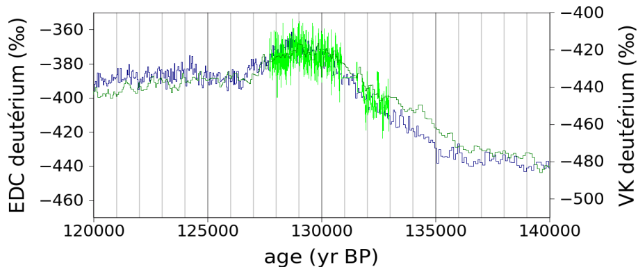
Fig. 8. EDC/VK isotopic phasing during termination II after volcanic synchronisation Blue: EDC deuterium record on its EDC3 age scale. Green: Vostok 3G deuterium record on the EDC3 age scale (after synchronisation, assuming 3G depths and 5G depths are synchronous). Light Green: Vostok 5G deuterium record on the EDC3 age scale (after synchronisation).
