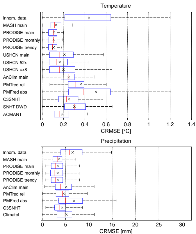
Fig. 3. Boxplot of the decadal CRMSE of the complete contributions, for temperature (top) and precipitation (bottom). For comparison the error metric for the inhomogeneous data is plotted at the top. The abscissa is the same as the one of Fig. 2 to emphasize the smaller errors and larger improvement over the inhomogeneous data for the decadal data. The conventions of the boxplots are explained in Fig. 2.
