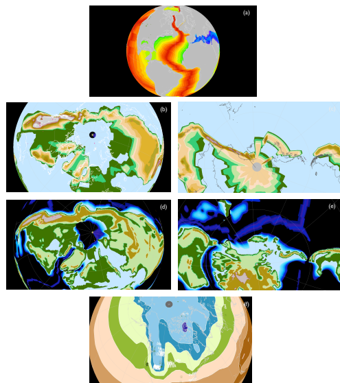
Fig. 1. Comparison of paleogeographic information used in the simulation with independent reconstructions from Mueller et al. (2008) via the freely available GPLATES software and via personal communication from Paul Markwick. In (a) a plate tectonic reconstruction for 55 mya from GPLATES including sea floor age is shown. This plate configuration is an excellent match to the land-sea distribution developed in Sewall et al. (2000) used in the simulations here (b) . The modern continental boundaries in their 55 mya positions as reconstructed by GPLATES are shown in (a–c) . The topography used in model is compared with the independently derived high resolution early Eocene topography of Markwick (based on Markwick, 1998) in (b–e) . In (f) an example of how the pointwise comparison of model and proxy records is performed is shown. Colors are modelled temperatures and the text indicates the abbreviated names of proxy localities. Based on modern latitude and longitudes the localities are rotated back to 55mya positions using GPLATES, thus enabling the best objective placement of the paleo-positions within the model's reference frame. As (f) shows, errors in paleo-position are unlikely to introduce large errors in inferred temperature except in regions with strong temperature gradients, i.e. in regions of strong elevation variation.
