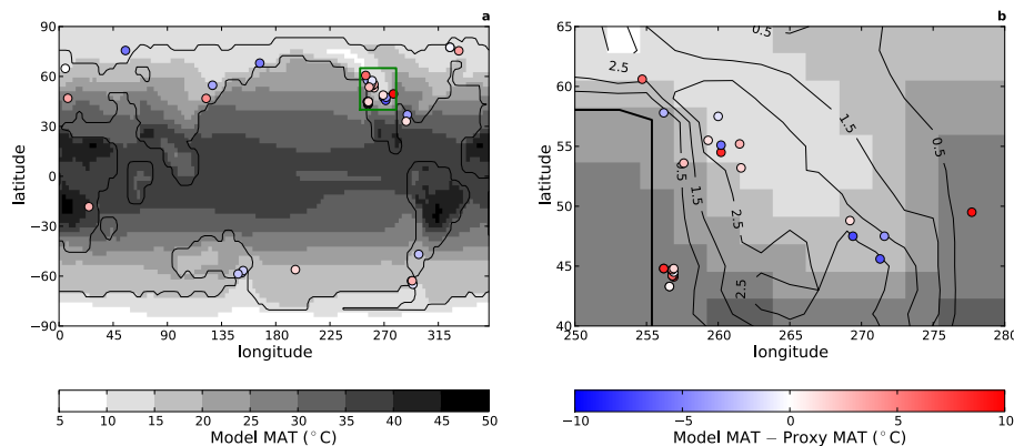
Fig. 5. Difference between modelled and reconstructed MAT as indicated by the color bar (on the right) overlain on the the model predicted temperatures (grey scale color bar on left).
