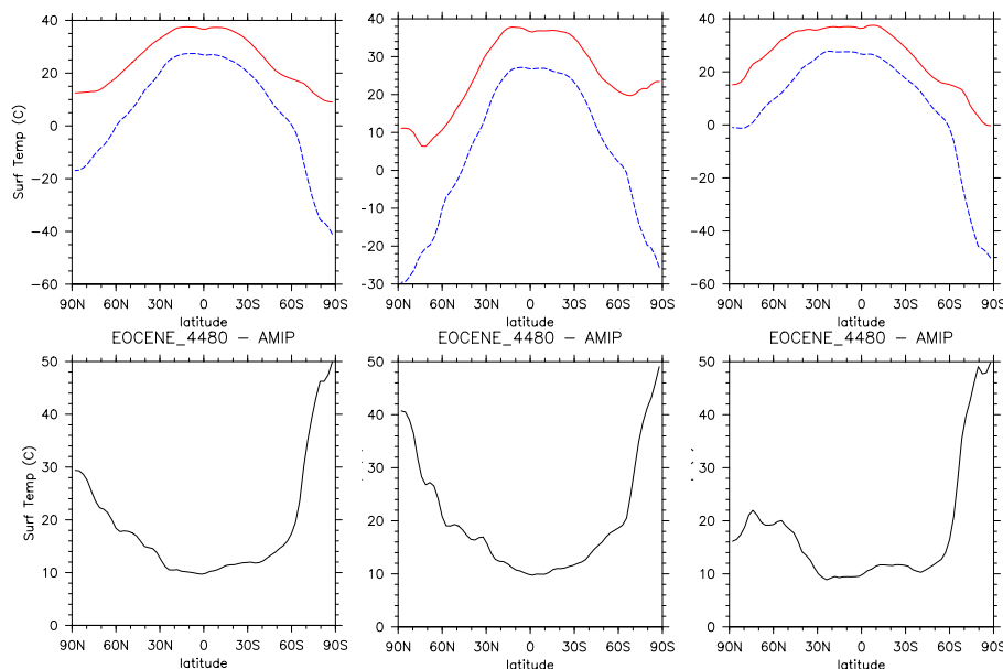
Fig. 2. Zonal mean surface temperature from the EOCENE-4480 (red) and modern (AMIP) simulations as described in the text. In the upper row, the annual (left) boreal winter (middle) and boreal summer (right) means are shown. In the lower row, the anomaly, EOCENE-4480 minus modern is shown.
