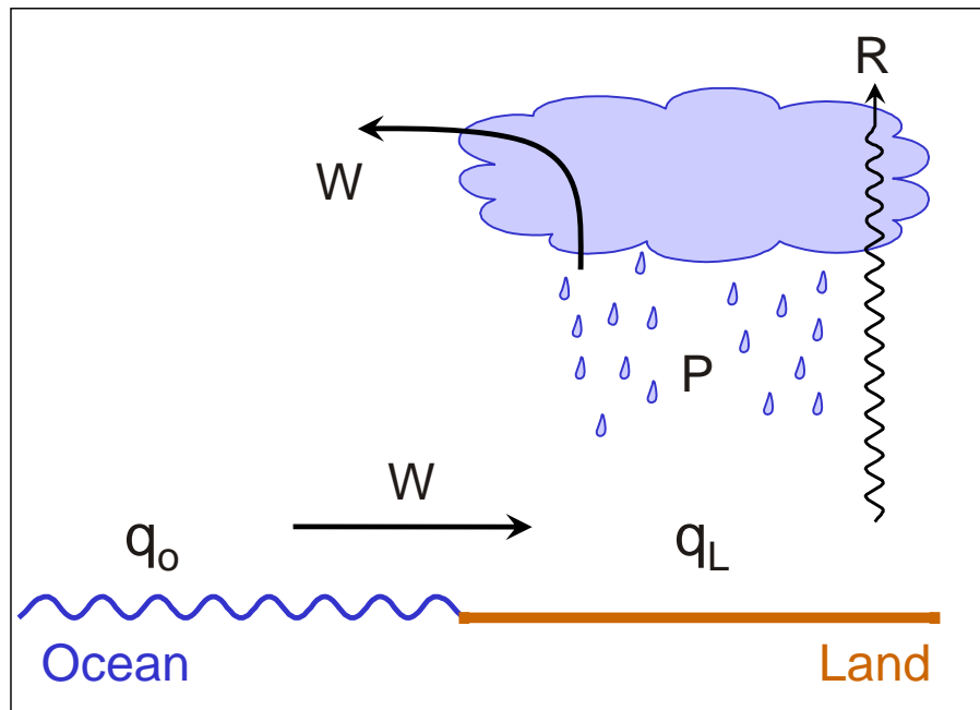
Fig. 1. Geometry of the conceptual model, illustrating wind W , precipitation P , net radiative flux R , and atmospheric specific humidity over land ( q_L ) and ocean ( q_o )
