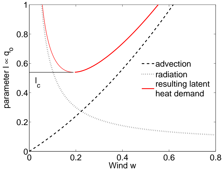
Fig. 5. Solution structure of the conceptual model as a function of the non-dimensional parameter l , which is proportional to specific humidity over the ocean, q_0 . For illustrative purposes, l is plotted on the y-axis. The latent heat demand (red line; bold part indicates the stable branch) results from heat loss due to net radiative flux (dotted) and advection of warm air out of the land region (dashed).
