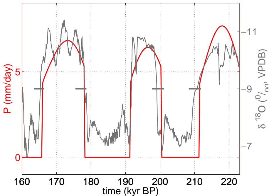
Fig. 10. Grey: Speleothem \delta^{18}\text{O} record from central China, used as EASM proxy for the penultimate glacial period, where more negative values indicate stronger rainfall (Wang et al., 2008). The record is smoothed with a 5-point running average, and dating errors ( \pm 2\sigma ) are shown for selected dates (grey horizontal bars). Red: Result of the conceptual model for EASM precipitation P in response to q_o variations driven by Northern Hemisphere ( 65^\circ\text{N} ) summer insolation, assuming a hysteresis of 0.5\text{ g kg}^{-1} width. For illustration, we set P to zero during periods when no monsoon circulation exists according to the model.
