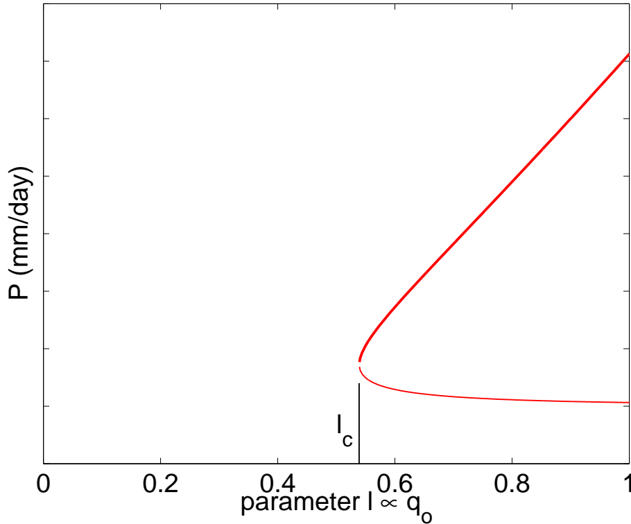
Fig. 7. As Fig. 6, but in terms of dimensional precipitation P . The shape of the solution is different than in terms of p because the relation between p and P depends on l . Units on the y-axis are arbitrary.
