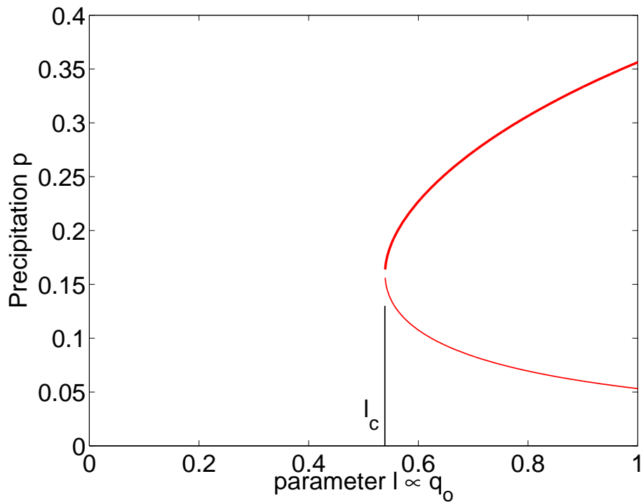
Fig. 6. As Fig. 5 (red line), but in terms of non-dimensional precipitation p , and organized with the control parameter l on the x-axis.
