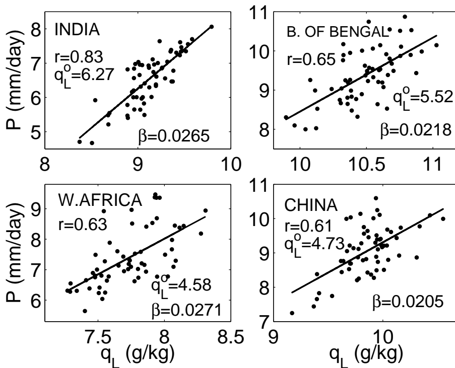
Fig. 4. Precipitation P versus specific humidity over land, q_L , from NCEP/NCAR reanalysis data. The black line shows the result of a linear regression, the correlation coefficient r is indicated, as well as the slope \beta (in \text{kg m}^{-2} \text{s}^{-1} ) and the offset in terrestrial humidity, q_L^0 (in \text{g kg}^{-1} ).
