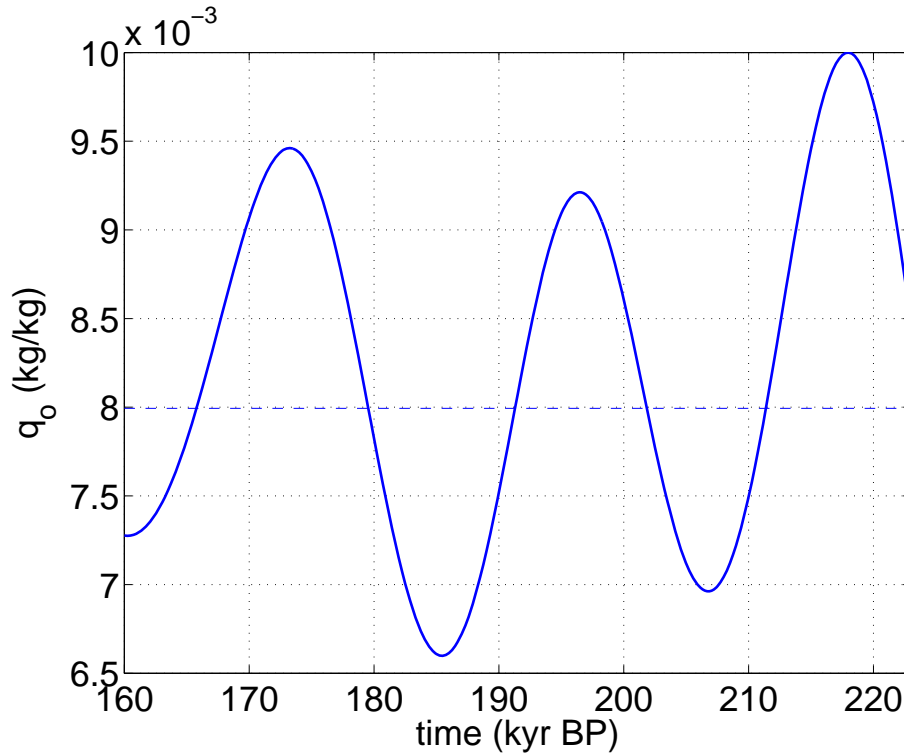
Fig. 12. Time series of q_0 used for the application of the conceptual model. q_0 is assumed to vary linearly with Northern Hemisphere ( 65^\circ\text{N} ) summer insolation. The horizontal dashed line marks q_0^c .
