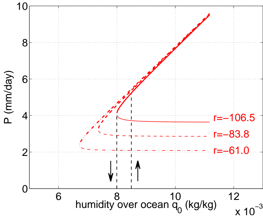
Fig. 11. Physical solution for EASM precipitation P from the conceptual model, for three different values of the non-dimensional parameter r : \overline{r(t)} (dashed), \overline{r(t)} + \sigma/2 (dot-and-dash), and \overline{r(t)} - \sigma/2 (solid), where r(t) is the estimate from NCEP/NCAR reanalysis data, and \sigma denotes a standard deviation. Bold lines indicate the upper, stable branch. The value \overline{r(t)} - \sigma/2 = -106.5 , which corresponds to a critical threshold q_0^c = 8.0 \text{ g kg}^{-1} , is used for the comparison of the model with EASM proxy data. Vertical dashed lines mark q_0^c and q_0^c + \Delta_q , where we choose \Delta_q = 0.5 \text{ g kg}^{-1} as the width of an assumed hysteresis that is thought to appear when the threshold is crossed from either side (illustrated by arrows).
