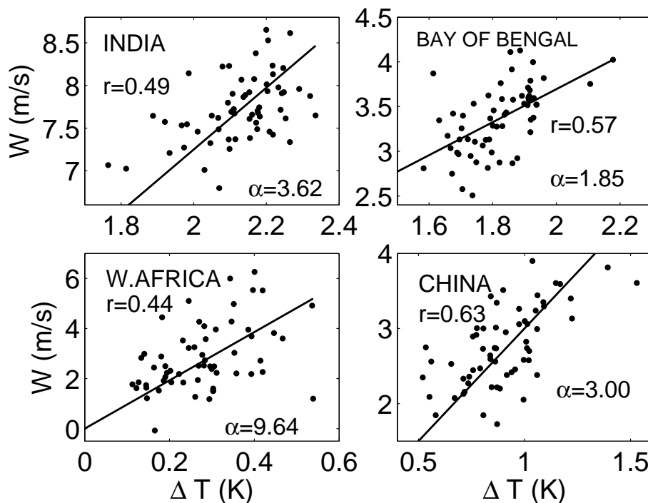
Fig. 3. Wind W versus temperature difference between land and ocean region, \Delta T , from NCEP/NCAR reanalysis data, for the major monsoon regions of India, the Bay of Bengal, West Africa, and China (East Asia; see Table 1). The correlation coefficient r is indicated, as well as the slope \alpha of a linear fit through the origin (black line).
