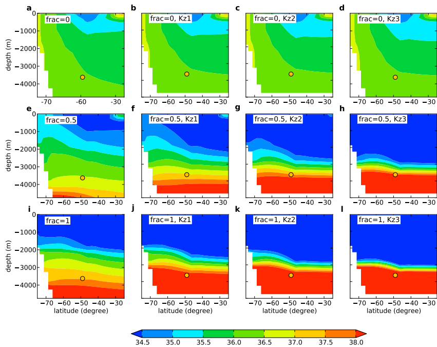
Fig. 2. Salinity distribution (permil) in the Atlantic ocean as simulated by the model. The dot is the data from Adkins et al., 2002 (Shona Rise, 49S, 3626 m).
