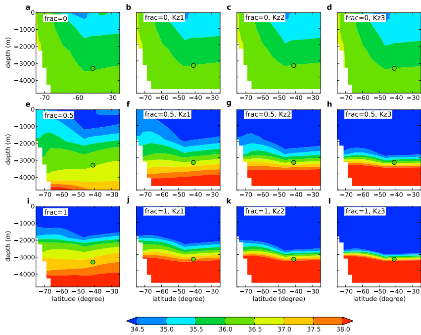
Fig. 1. Salinity distribution (permil) in the Pacific ocean as simulated by the model. The dot is the data from Adkins et al., 2002 (Chatham Rise, 41S, 3290 m).
