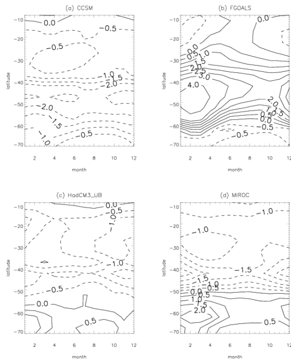
Fig. 1. The difference in SST (K) between the HadSST2 dataset and each of the available PMIP2 models control (PI) runs - (a) CCSM, (b) FGOALS, (c) HadCM3_UB and (d) MIROC.
