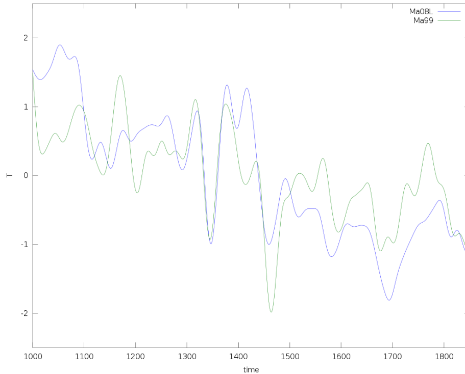
Fig. 2. The Ma08L and Ma99 reconstruction (smoothed)
