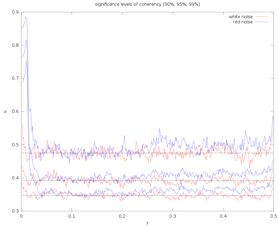
Fig. 1. Estimating significance levels
