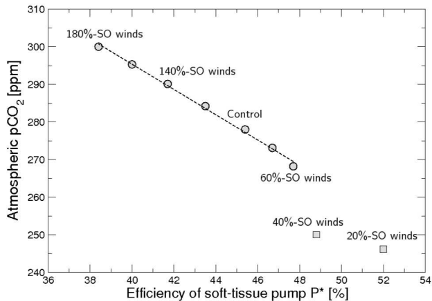
Figure 1: Ocean ventilation experiments: Quasi-linear relation between simulated atmospheric CO 2 and the efficiency of the soft-tissue pump P* (Ito and Follows (2005)) for the ventilation states with active NADW formation (circles). The linear relation is perturbed when NADW formation is shutdown in response to strongly reduced windstress in the Southern Ocean (rectangles).
