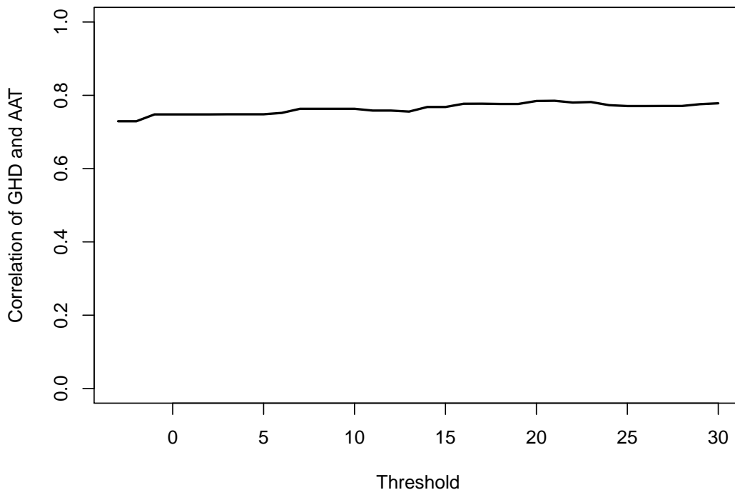
Fig. 4. GHD-AAT correlation. All years with a GHD- first frost difference less than the threshold are omitted prior correlation
