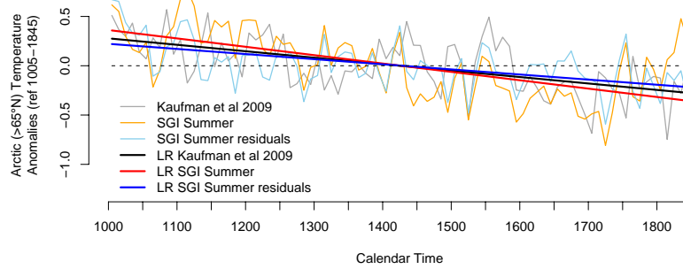
Fig. 8. Comparison between the Arctic summer temperature reconstruction provided by Kaufman et al. (2009) (grey and black lines) and SGI. The orange and red lines show the summer mean in SGI. The blue lines show the residuals calculated as the summer temperature time series in SGI, minus the signatures of TSI and CO 2 (equivalent to the \varepsilon_3 residuals in Eq. 3). The grey, orange and light blue thin lines represent the ten-year smoothed time series of Kaufman et al. (2009), SGI summer mean and SGI summer residuals respectively. The thick black, red and blue lines show the linear regressions associated with the summer temperature time series of Kaufman et al. (2009), SGI summer mean and SGI summer residuals, respectively.
