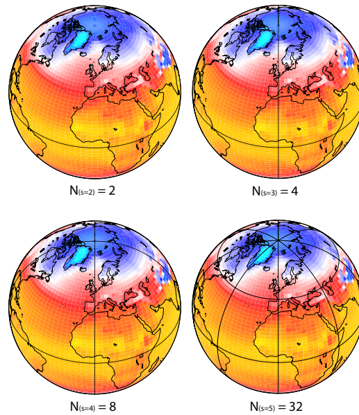
Fig. 4. Second to fifth step of the algorithm cutting the surface of the Earth in individual areas. N is the number of areas delimited by the black straight lines, and s the step in the algorithm. The surface temperature is averaged over all the individual areas to calculate the SNR.
