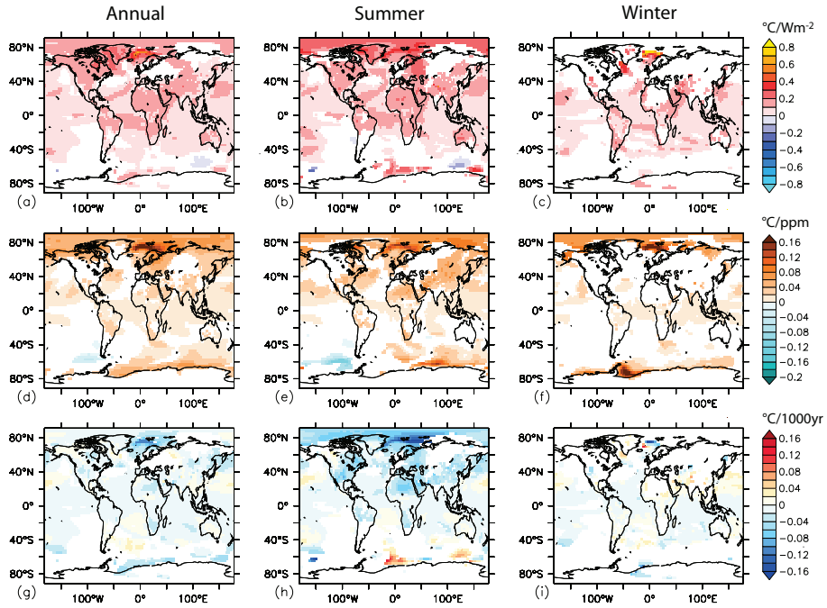
Fig. 6. First order sensitivity of the temperature in SGI to TSI variability estimated by C_1^{BV} expressed in ^{\circ}\text{C}/\text{Wm}^{-2} (a, b, c), to \text{CO}_2 by C_2^{BV} expressed in ^{\circ}\text{C}/\text{ppm} (d, e, f), and slope of the \varepsilon_3 residuals corresponding to C_3 expressed in ^{\circ}\text{C}/1000\text{yr} (g, h, i). Those coefficients are calculated for annual (a, d, g), summer (b, e, h) and winter (c, f, i) averages. The white areas represent the grid points where the coefficients are not significant at 99.5% (Student t-test).
