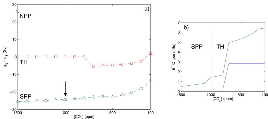
Fig. 7. Same as Fig. 6 but with the inception temperature of ice increased to 3^\circ\text{C} : (a) Simulated bifurcation diagram showing pattern and strength of the MOC for different initial states: NPP (circles), TH (squares) and SPP (triangles). The arrow denotes the CO_2 concentration at which the small density perturbation in the northern surface box was applied. (b) Simulated \delta^{18}O profile when a density perturbation is applied to the SPP MOC in the northern surface box at a CO_2 concentration of 1000 ppm. The \delta^{18}O profile is separated into the contribution due to changes in ice volume ( \delta_w , blue) and the total signal with the added effect of deep sea temperature changes ( \delta_c , green). The first shift in \delta_c represents the transition in the MOC from the SPP to the TH state, the second shift represents Antarctic ice growth.
