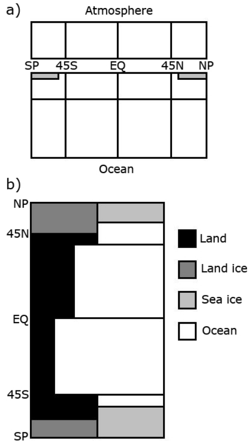
Fig. 1. Box model (a) meridional cross section with shaded regions representing sea ice cover; (b) top view. Adapted from Gildor and Tziperman (2001). In our study, sea ice is not present.
