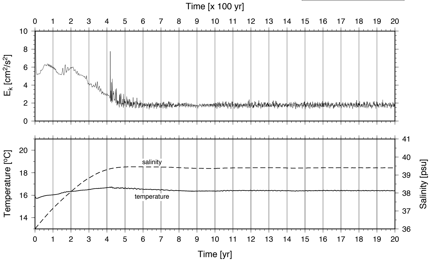
Figure R6. 2-kyr integration.
