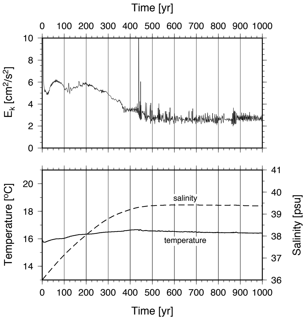
Figure R1. Wind stress added.
