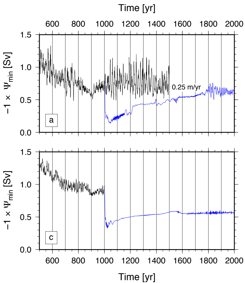
Figure R3. Wind stress added.
