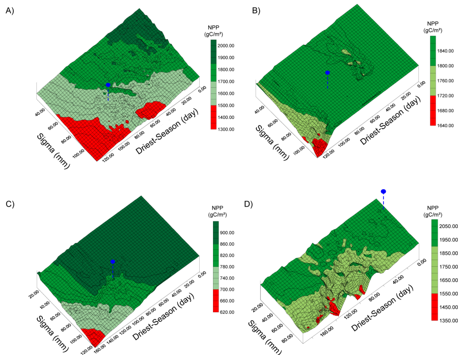
Fig. 6. Sensitivity test in a tridimensional representation ( \text{gC m}^{-2} \text{yr}^{-1} ), number of consecutive dry days, sigma of the prescribed precipitation distribution), at Ngamakala for tropical trees (A) and tropical grasses (B) , and at Kuruyange (C) and at Lake Victoria (D) for tropical grasses. Dashed line with solid circle corresponds to NPP value obtained with the modern precipitation distribution.
