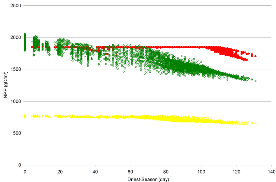
Fig. 4. Evolution of the NPP for different PFTs, as a function of the variable driest season (number of consecutive days) for Ngamakala (400 m). Solid circle, tropical/warm grass PFT (trg); Open lozenge, tropical raingreen trees PFT (trt); Open triangle, woody desert plant type C3 and C4 PFT (wod).
