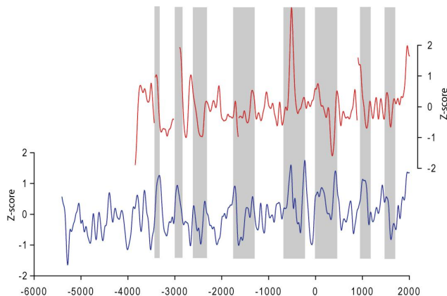
Fig. 3. A comparison between the Torneträsk (blue) and Jämtland (red) tree-ring width chronologies. Both records have been RCS standardized (see text) and transformed into Z-score values, showing centennial variability. Interpreted synchronous periods are shown in grey.
