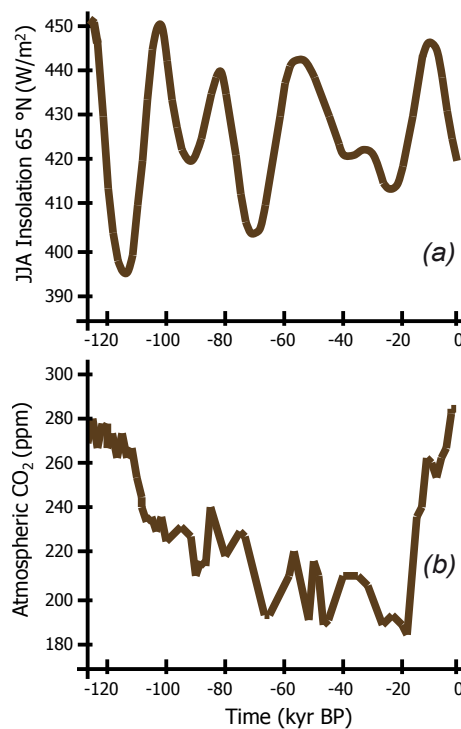
Fig. 1. Forcing factors: (a) summer insolation at 65° N ( \text{W}/\text{m}^2 ) (Berger, 1978); (b) atmospheric \text{CO}_2 concentration (ppm) (Petit et al., 1999).
