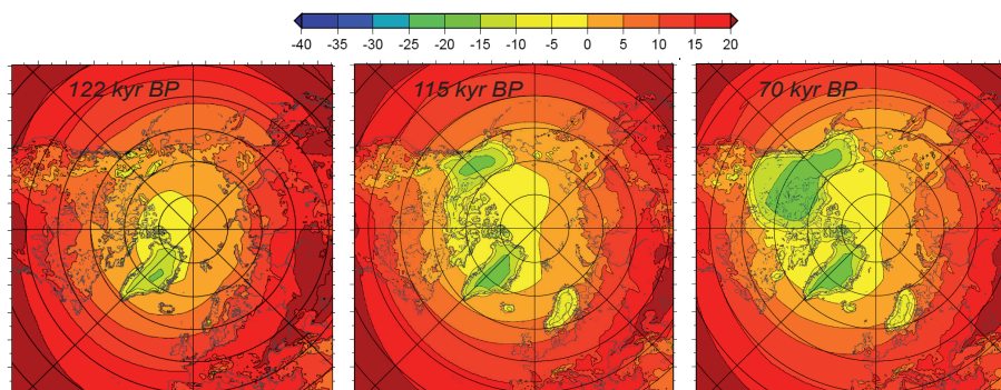
Fig. 3. Simulated average summer surface air temperatures (JJA) at different key periods (in °C): 122 kyr BP (left panel), 115 kyr BP (middle panel) and 70 kyr BP (right panel). These periods represent the starting phase of pronounced cold episodes characteristics of the last climatic cycle.
