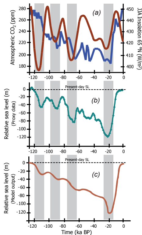
Fig. 5. (a) Forcing factors: summer insolation at 65° N ( \text{W/m}^2 ) (Berger, 1978; red line) and atmospheric \text{CO}_2 concentration (ppm) (Petit et al., 1999; blue line); (b) Relative sea level (m) inferred from benthic isotopic records (Waelbroeck et al., 2002; green line); (c) Simulated sea level evolution (m) (orange line).
