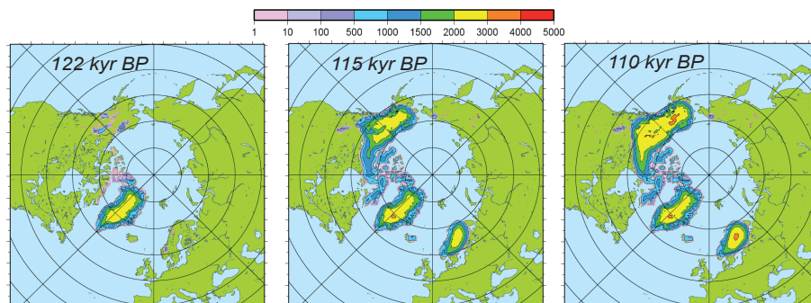
Fig. 2. Simulated ice thickness (in m) at different key periods during glacial inception: 122 kyr BP (left panel), 115 kyr BP (middle panel), 110 kyr BP (right panel).
