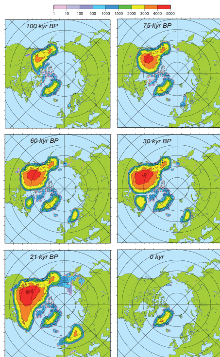
Fig. 4. Simulated ice thickness (in m) at different key periods: 100 kyr BP, 75 kyr BP, 60 kyr BP, 30 kyr BP, 21 kyr BP, 0 kyr BP.
