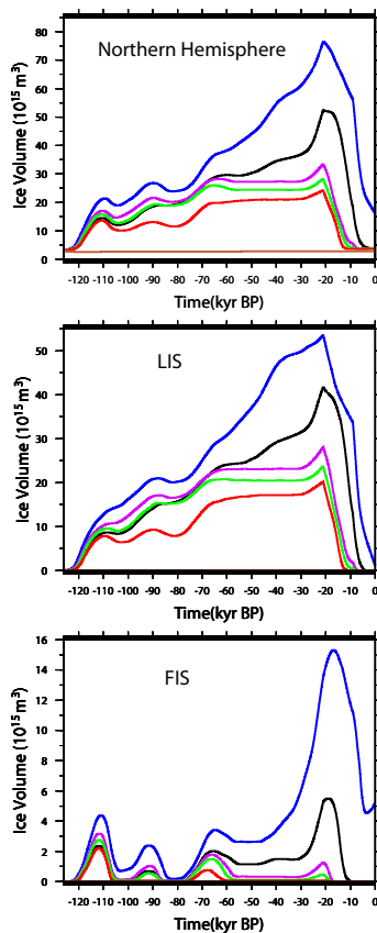
Fig. 6. Temporal evolution of the simulated ice volumes for the NH (top panel), the LIS (middle panel) and the FIS (bottom panel). The different curves correspond to the six different 126-kyr transient experiments: BSL (black line), CO 2 -200 (blue line), CO 2 -235 (purple line), CO 2 -250 (green line), CO 2 -280 (red line), INSO-126 (brown line).
