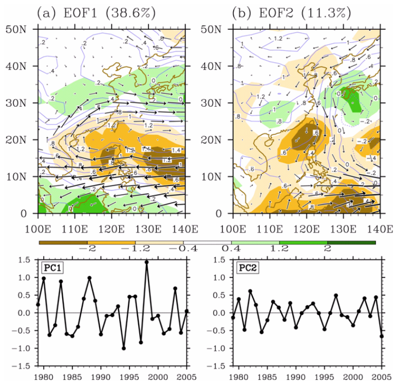
Fig. 2. Spatial patterns (upper panels) and their corresponding principle components (lower panels) of the first two MV-EOF modes of the EASM. Shown in the upper panels are anomalous JJA 850 hpa winds (vectors in units of m/s), precipitation (color shading in units of mm/day), and sea-level pressure (contours in units of hPa). Precipitation was derived from GPCP and other variables were derived from NCEP reanalysis-2.
