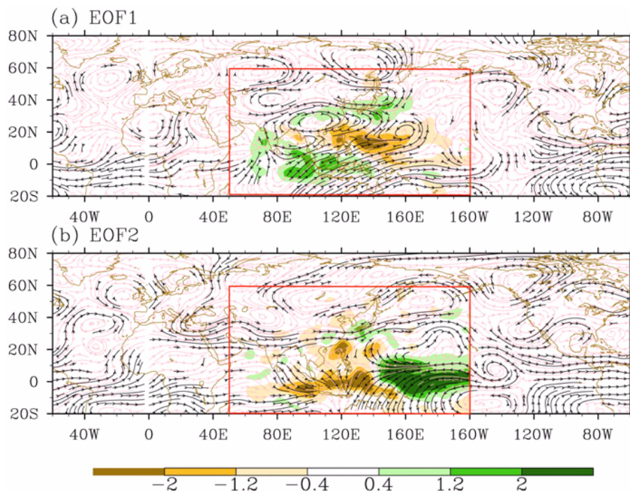
Fig. 4. Teleconnection patterns associated with the first two MV-EOF modes of interannual variability. Shown are the JJA precipitation anomalies (color shading in units of mm/day) and 200 hpa anomalous streamlines (pink lines) over the North Hemisphere. The anomalies were obtained by regression with respect to the first two principle components, respectively. The dark streamlines are statistically significant at the 95% confidence level.
