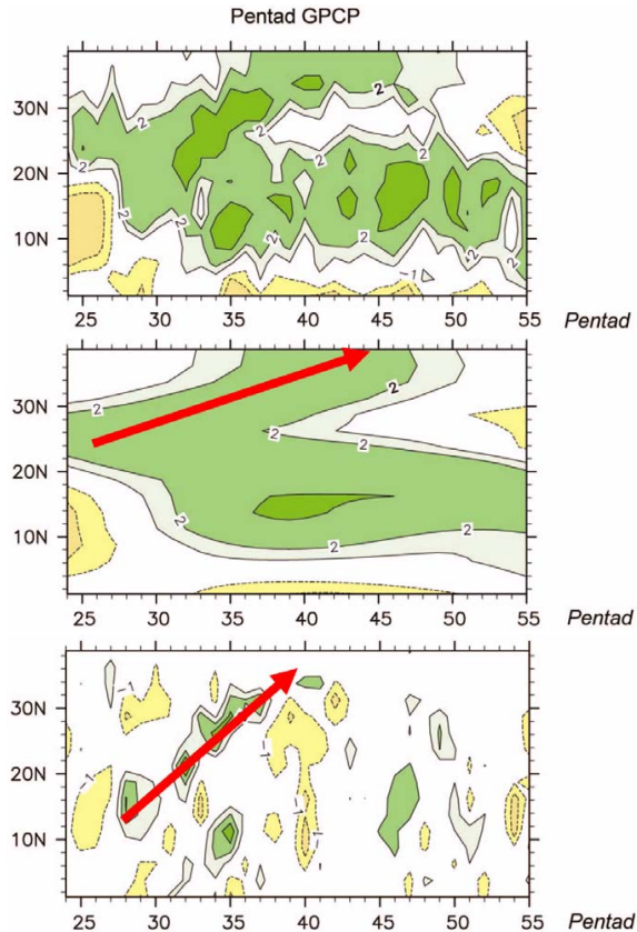
Fig. 5. The upper panel shows climatological pentad mean annual cycle of precipitation (contour interval is mm/day) as a function of latitude (ordinate) and Julian pentad (abscissa). The middle and lower panels are the same as in the upper panel except for the slow and fast annual cycle, respectively. The definitions of the slow and fast annual cycle are referred to the text. The red arrows indicate the seasonal migration of the subtropical rain band as seen in the slow and fast annual cycles.
