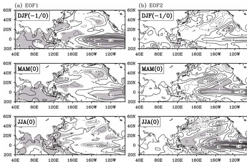
Fig. 3. Evolution of SST anomalies associated with the two MV-EOF modes. These patterns were obtained by regressing with respect to the first two principal components of the MV-EOF analysis for three consecutive seasons: DJF(-1/0), MAM(0) and JJA(0), where “0” denotes the year concurring with the EA-WNP leading modes. “-1” denotes the year precedes year 0. Grey shadings indicate areas where the anomalies are statistically significant at the 95% confidence level. The SST data are from NOAA Extended Reconstructed Sea Surface Temperature Version 2.
