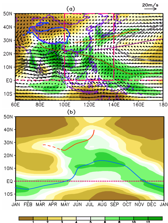
Fig. 1. (a) Climatological summer (JJA) mean precipitation (color shading in mm/day) and 850 hPa winds (vectors in units of m/s). The Meiyu belt (brown line), WNPSH ridge (purple line) and WNP monsoon trough (dark brown line) have been outlined along with the Tibetan Plateau 3000 m contours (dark blue line). (b) Climatological monthly mean rainfall as a function of latitude (ordinate) and calendar month (abscissa). The precipitation is averaged over the EA sector between 110° E and 130° E. The ITCZ and EASM rain belt (the subtropical frontal rain belt) have been outlined by blue and red lines, respectively. Precipitation was derived from GPCP and other variables were derived from NCEP reanalysis-2.
