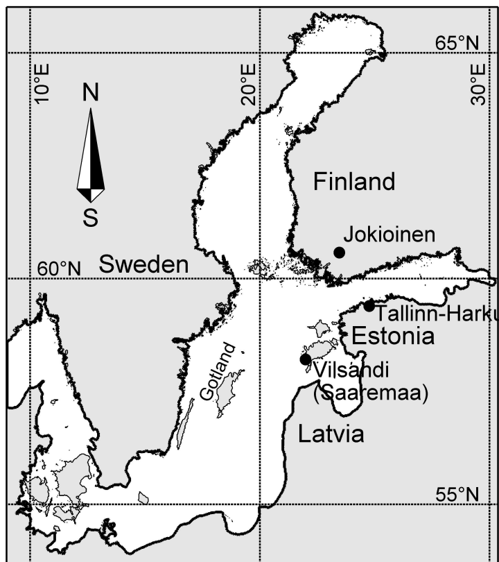
Fig. 1. Location scheme of the Baltic Sea, Tallinn-Harku Aerological Station, Jokiainen Observatory, and the Island of Vilsandi.
