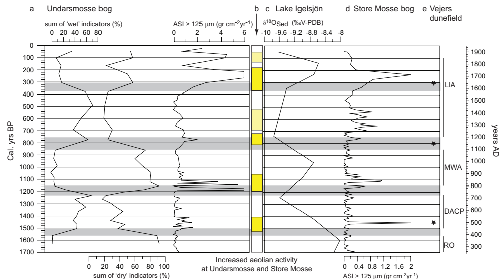
Fig. 3. (a) Data from Undarsmossen bog, showing humidity fluctuations as reconstructed by testate amoebae analysis, with an alternating dominance of wet and dry indicators. Curves are based on the taxa presented in Fig. 2 and Table 1. Grey shading indicates transitional phases between relatively stable hydrological conditions as reconstructed by testate amoebae. Also shown are ASI variations from the same core for grainsizes >125\ \mu\text{m} . (b) Summary of ASI data from Undarsmossen and Store mosse bogs (curve d). Yellow boxes indicate the timing and duration of increased aeolian activity at both sites. Light yellow boxes represent increased aeolian activity mainly recorded at one of the sites. (c) Effective humidity changes as recorded by Hammarlund et al. (2003) and Seppä et al. (2005). This proxy is comparable to the wetness indicators at this study site (Fig. 3a) and shows a similar pattern. (d) ASI results from Store Mosse bog. Comparison to the ASI record from Undarsmossen bog shows that the two records are highly similar. (e) Stars indicate the onset of dune formation at Vejers dunefield (Fig. 1), interpreted as a proxy for westerly storm activity and sand erodibility (Clemmensen et al., 2001; Clemmensen and Murray, 2006).
