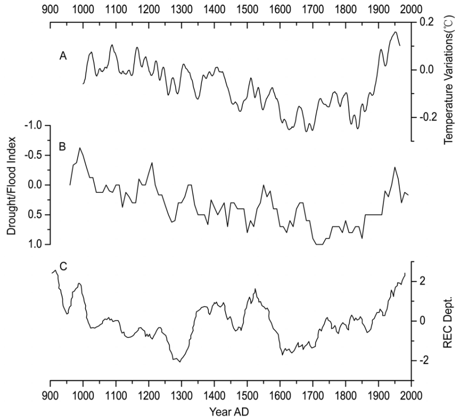
Fig. 5. Comparison of D/F series of Longxi ( B ), Northern Hemisphere temperature ( A ) (Crowley, 2000) and precipitation reconstructed series of Dulan ( C ) from tree ring after 40-year moving average (REC, the reconstructed curve) (Liu et al., 2006).
