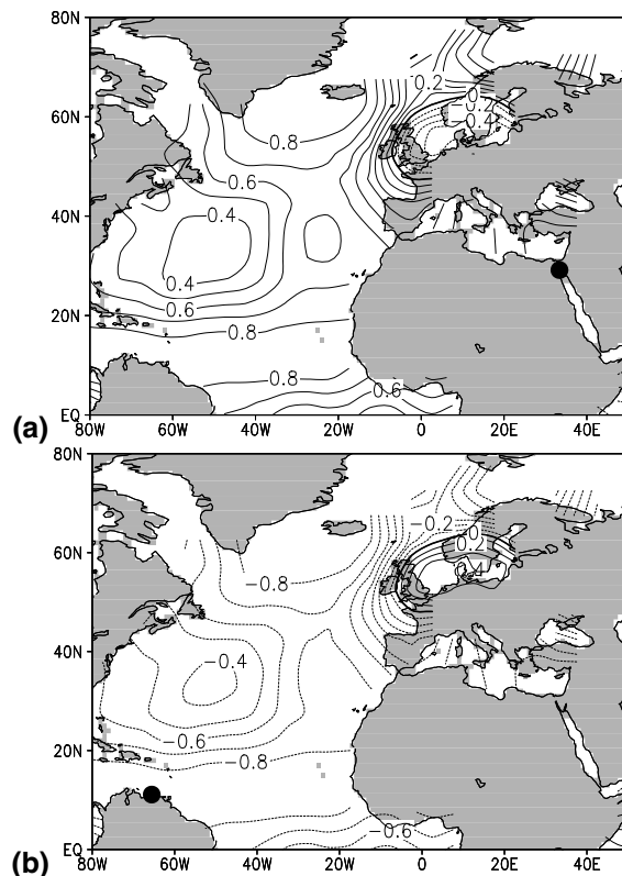
Fig. 2. Correlation map between gridded North Atlantic sea surface temperature (Mann et al., 1998) and proxy time series from (a) northern Red Sea Felis et al. (2000) and (b) Cariaco Basin (Black et al., 1999) for the period 1750–1980. Absolute correlation values exceeding \pm 0.65 fit the 90% confidence interval. Prior to correlation the data is detrended, normalized and Fourier filtered in the 50 years to 100 years frequency band. The proxy locations are indicated by circle, respectively.
