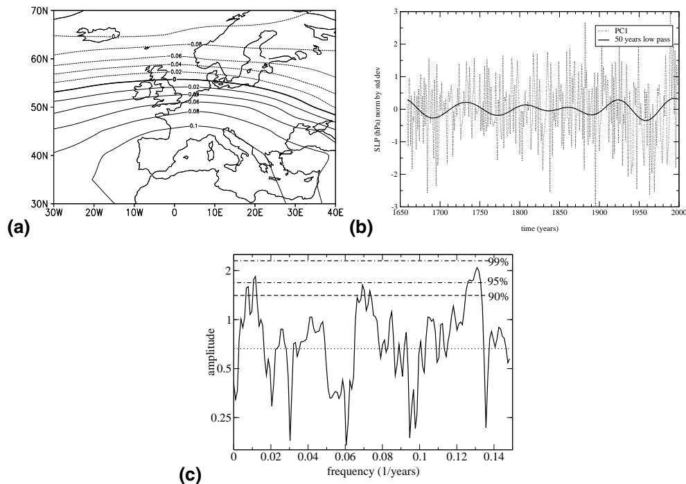
Fig. 3. EOF analysis of gridded sea level pressure data (Luterbacher et al., 2002) covering the period 1659–2000. (a) EOF1 explaining 46% of the variance. (b) Principal component of EOF1 in raw (dotted) and 50 year low pass filtered (solid) version. (c) Spectra based on white noise null hypothesis, with lines indicating median and significance levels.
