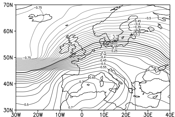
Fig. 5. Correlation map between proxy time series from Cariaco basin (Black et al., 1999) and SLP reconstruction data over North Atlantic (Luterbacher et al., 2002) covering 332 years starting from 1659. Correlation values exceeding \pm 0.65 fit the 95% confidence interval. All data is detrended, normalized and filtered in the band of 50 to 100 years prior to the analysis.
