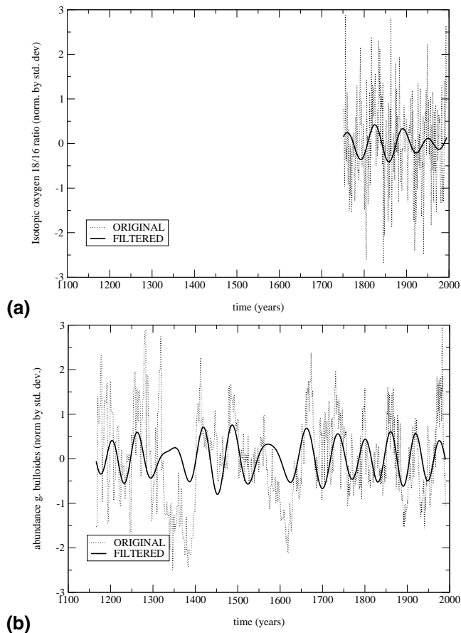
Fig. 1. Time series from (a) a coral (winter data) from the northern Red Sea (Felis et al., 2000) and (b) from a sediment core in Cariaco Basin (Black et al., 1999) indicate multidecadal variations. The data is detrended, normalized and shown in raw and 50–100 year band pass filtered version.
